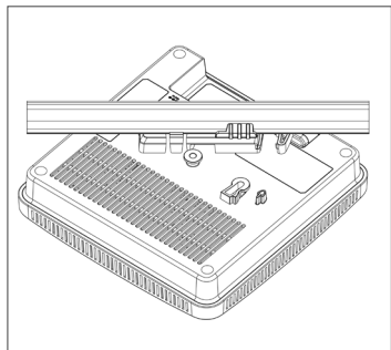
3. Place the first mounting post on the rear-side of the AP on to the lower notch of the bracket.
