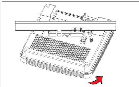
4. Rotate the AP such that the center mounting post fits in to the center notch on the bracket.
