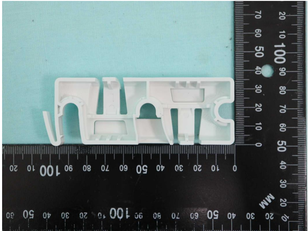
Bracket wall mount (O-235, O-235E)
