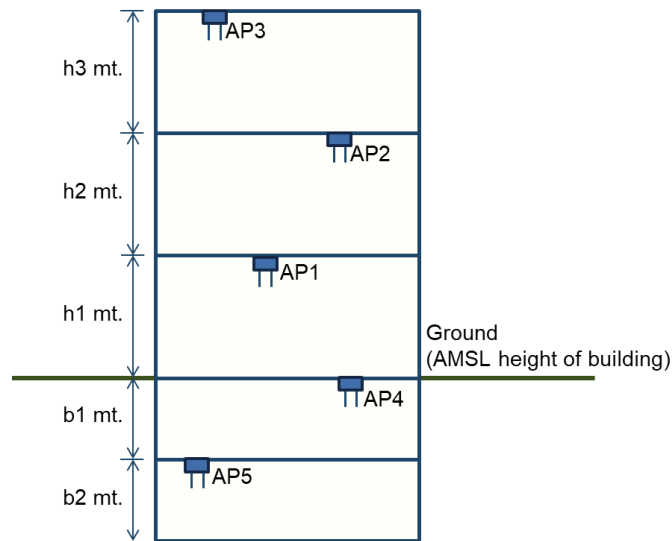
AP height estimation within a building
