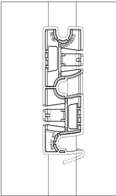
2. Rotate bracket to snap on to T-Grid.
