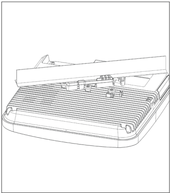
3. Place the first mounting post on the rear-side of the AP on to the lower notch of the bracket.
