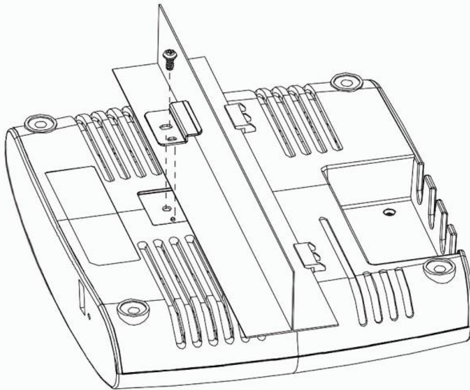
Figure 3-2 Wall Mounting
