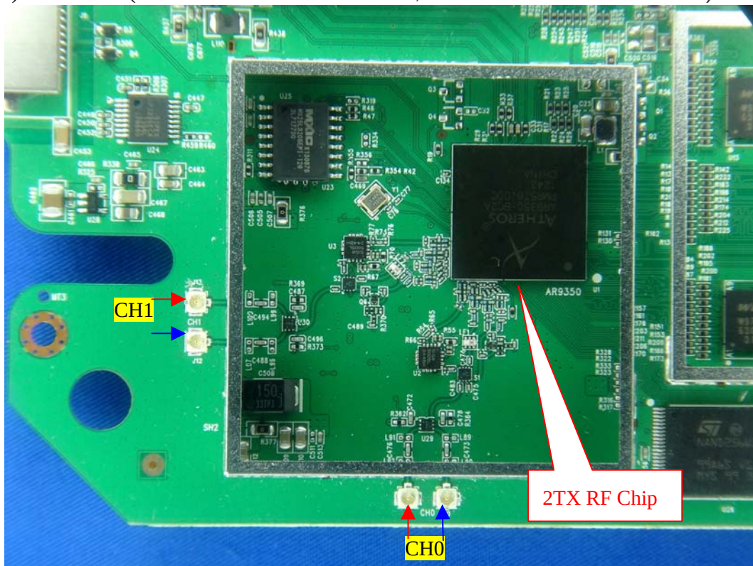
(20) EUT Photo (“Red” means external antenna, “Blue” means internal antenna)
