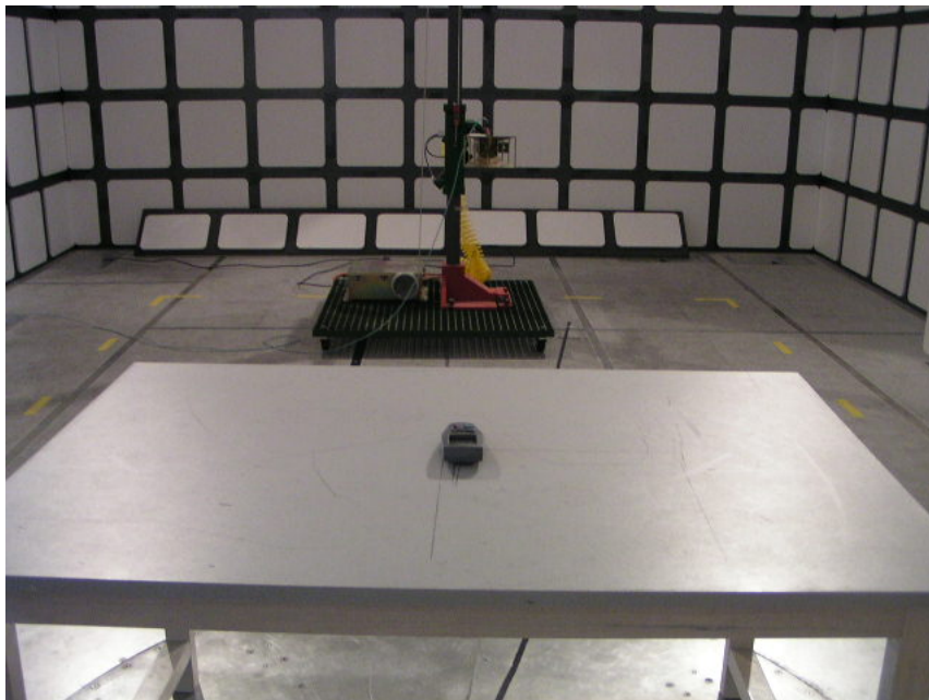
Radiated Emission - Rear View (Above 1GHz)
