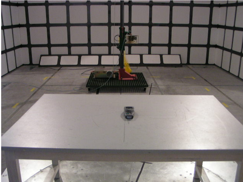
Radiated Emission - Front View (Above 1GHz)
