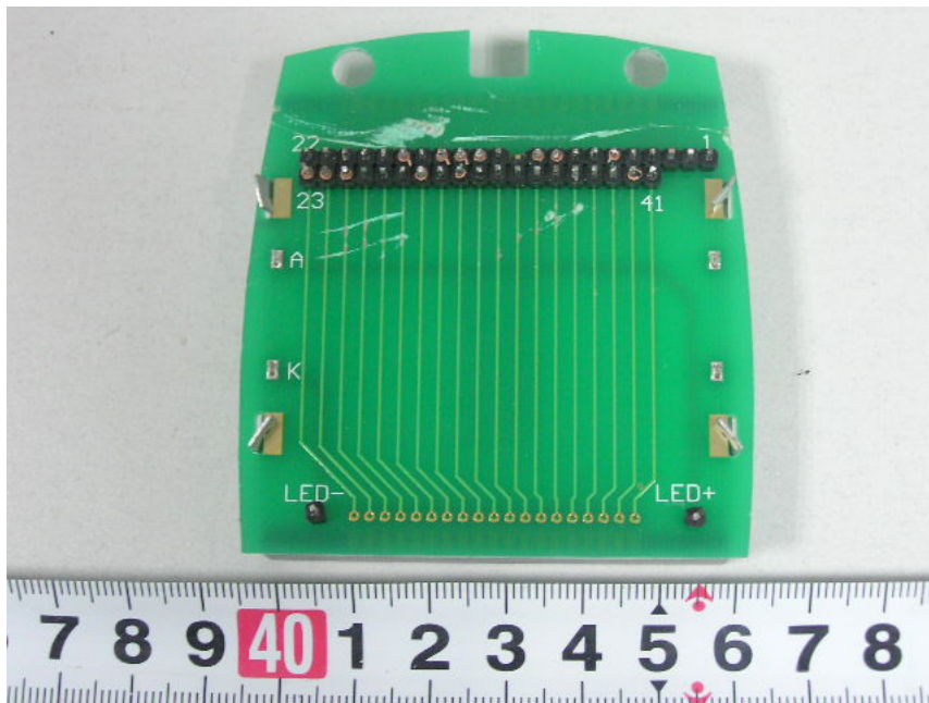
EUT – LCD Module Front View
