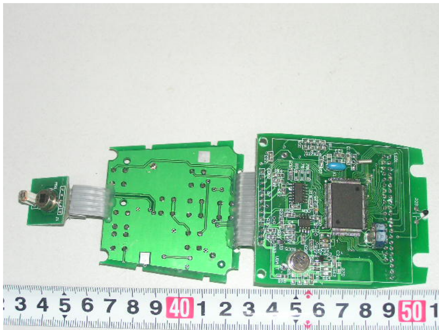
EUT – Main PCB Front View
