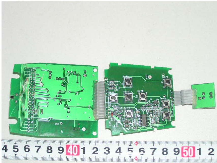
EUT – Main PCB Rear View
