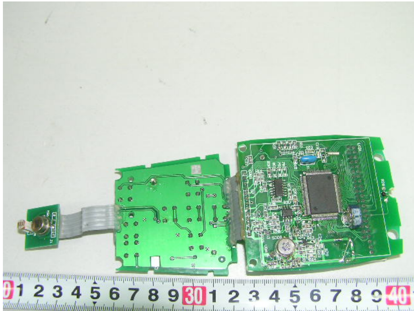
EUT – All Module Rear View
