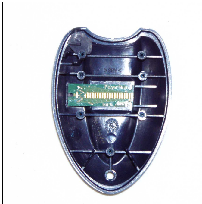
General view, PCB removed (upper side)
