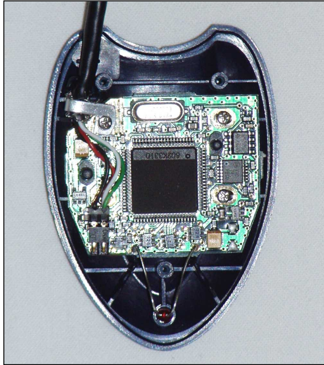
General view, cover opened (upper side)
