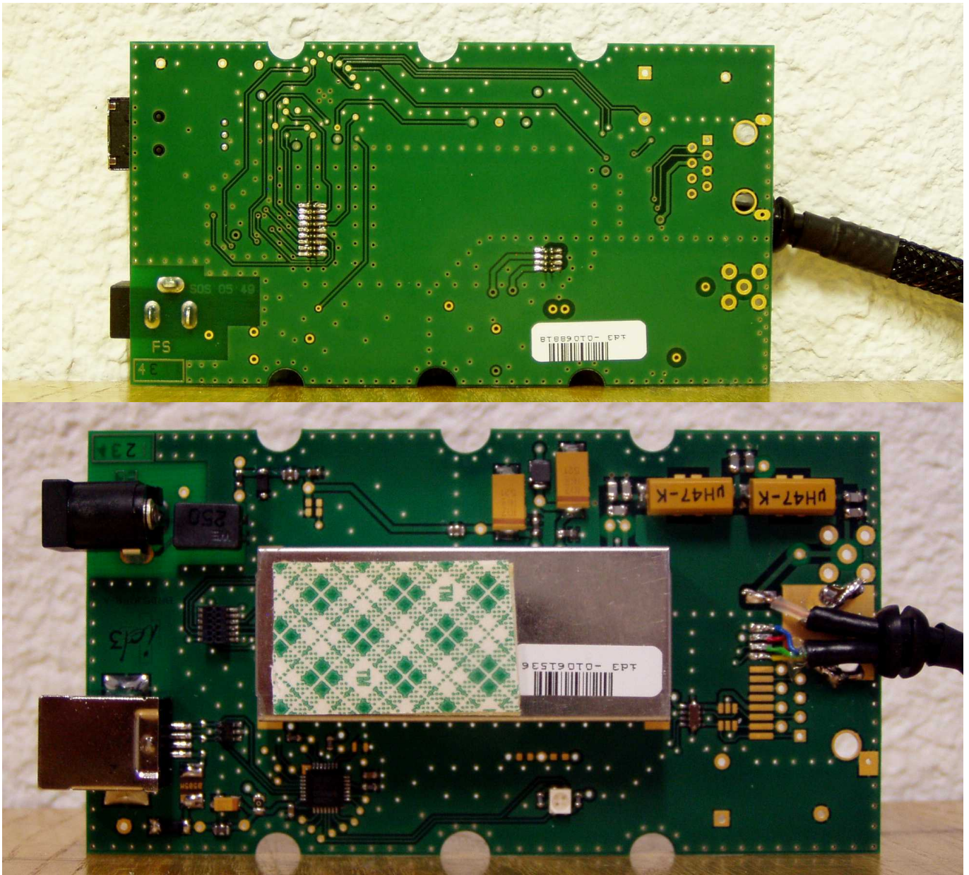
PCB view of the reader
