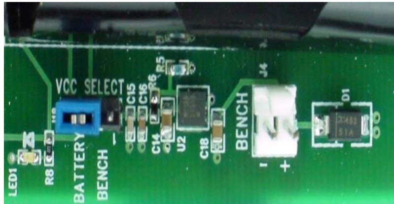
Figure 3-2. Jumper Set for Battery Supply
