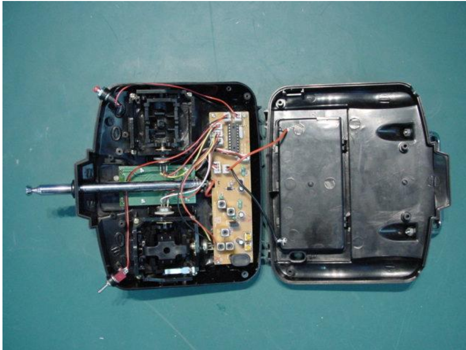
Photo 4 PCB photo
