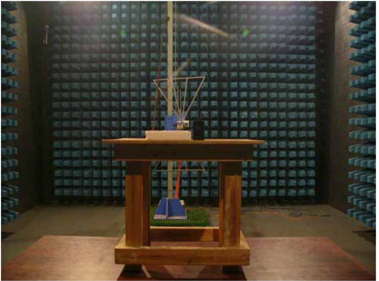
Photo for testing setup
