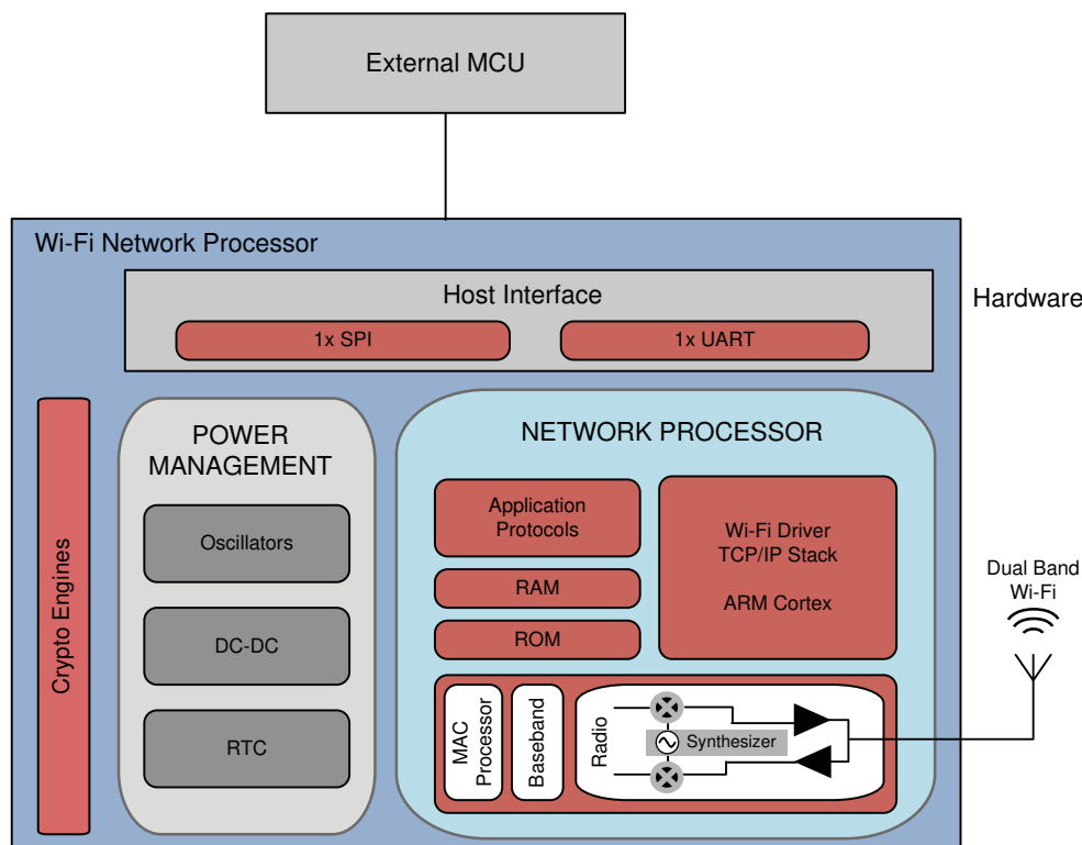
Figure 4-2. CC3135 Hardware Overview
