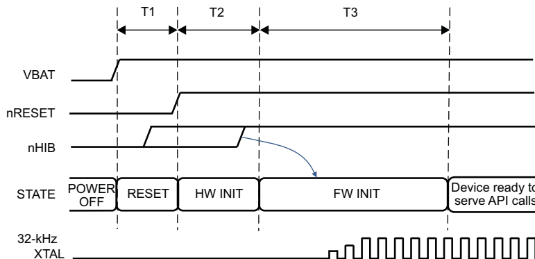
Figure 7-6. First-Time Power-Up and Reset Removal Timing Diagram
