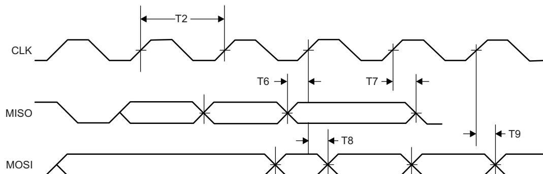
Figure 7-9. Host SPI Timing
