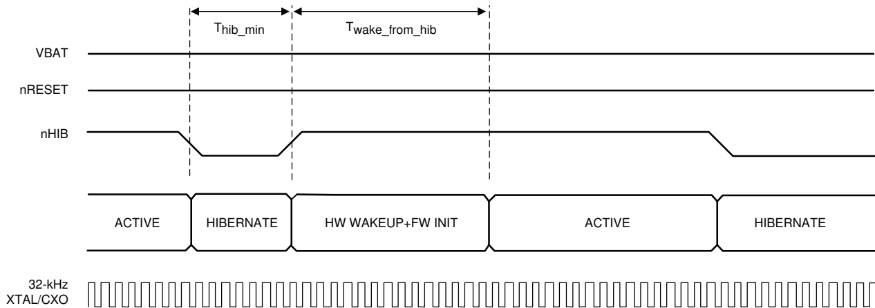
Figure 7-7. nHIB Timing Diagram
