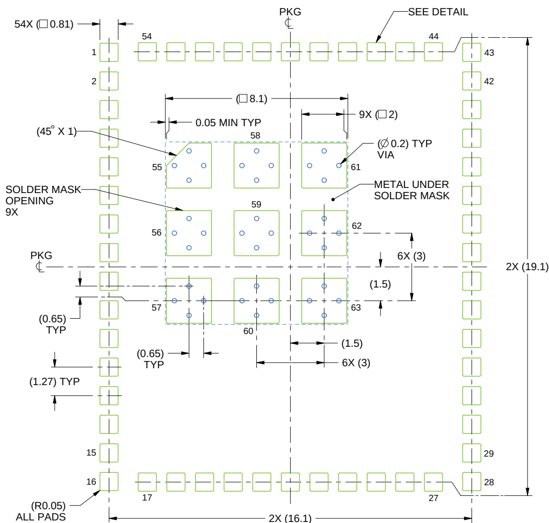
LAND PATTERN EXAMPLE SOLDER MASK DEFINED SCALE:6X
