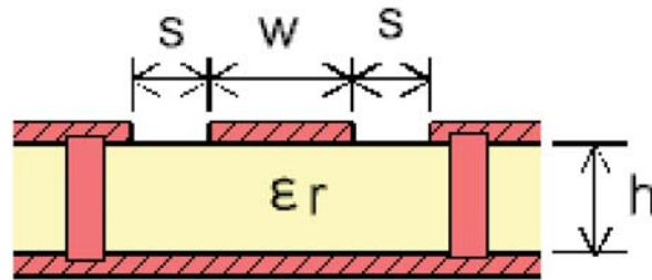
Figure 9-6. Coplanar Waveguide (Cross Section)
