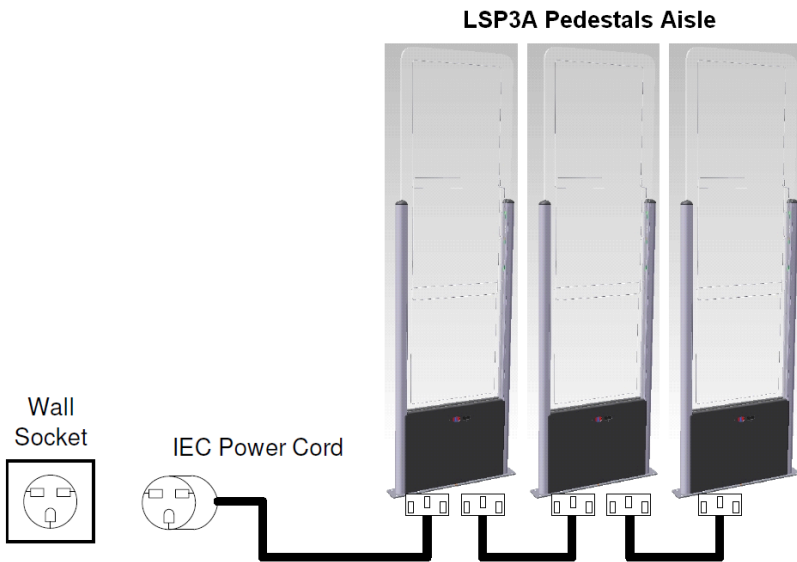
Figure 4.1: Safety Electrical Installation Using Power Cord
