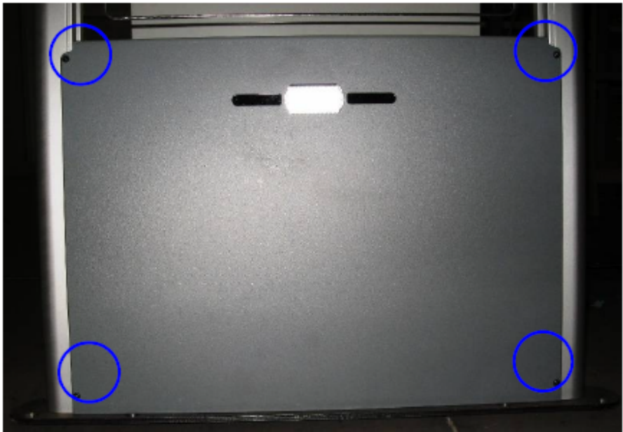
Figure 4.11: LSP3A-LR Clear Bottom Plastic Cover (4 screws)
