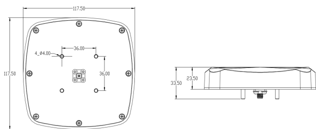
XC-AF802-BUS-A Type Antenna appearance dimension drawing
