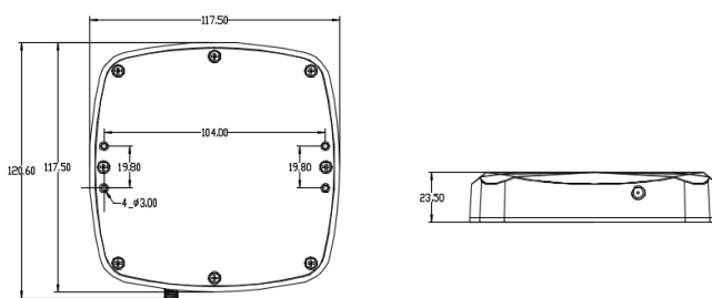
XC-AF802-BUS-B Type Antenna appearance dimension drawing
