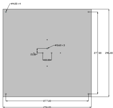
XC-AF618 Type antenna appearance dimension drawing
