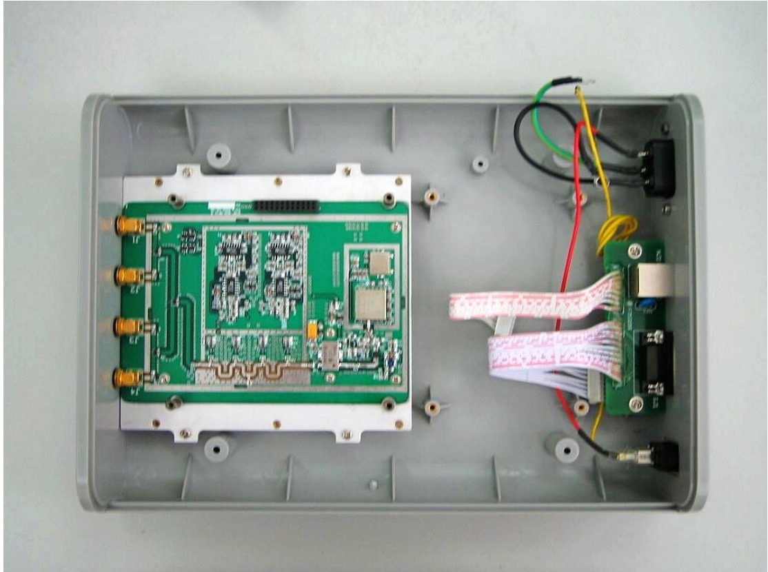
Internal of EUT-4
