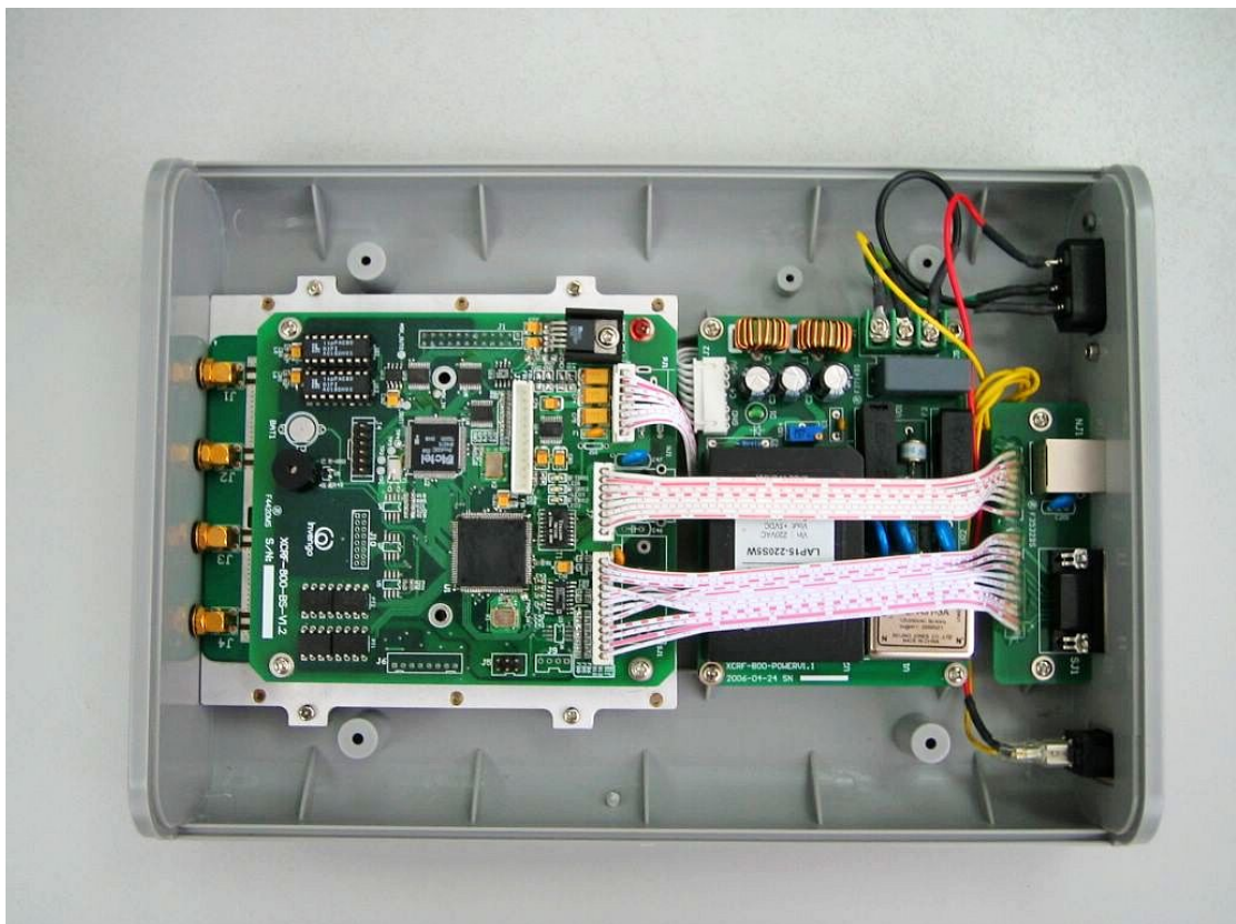
Internal of EUT-2
