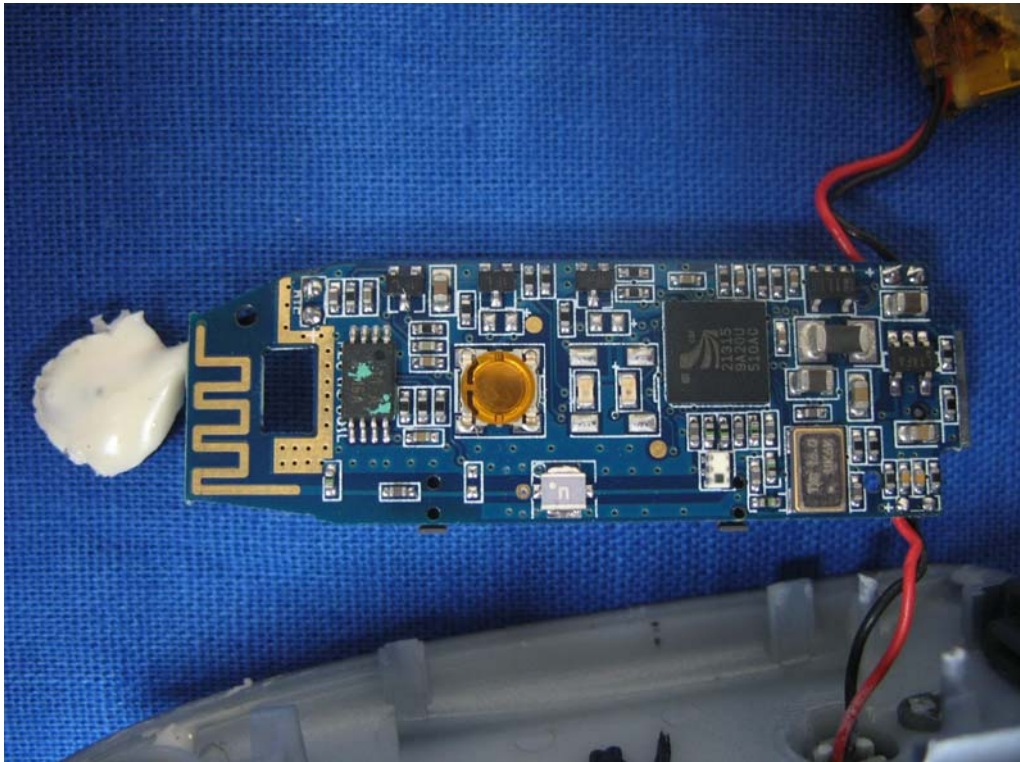
(3) EUT Photo (M/N: BTHS106)
