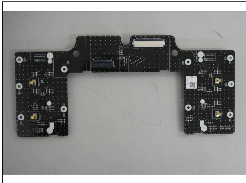
Bottom view of Key_2 PCB
