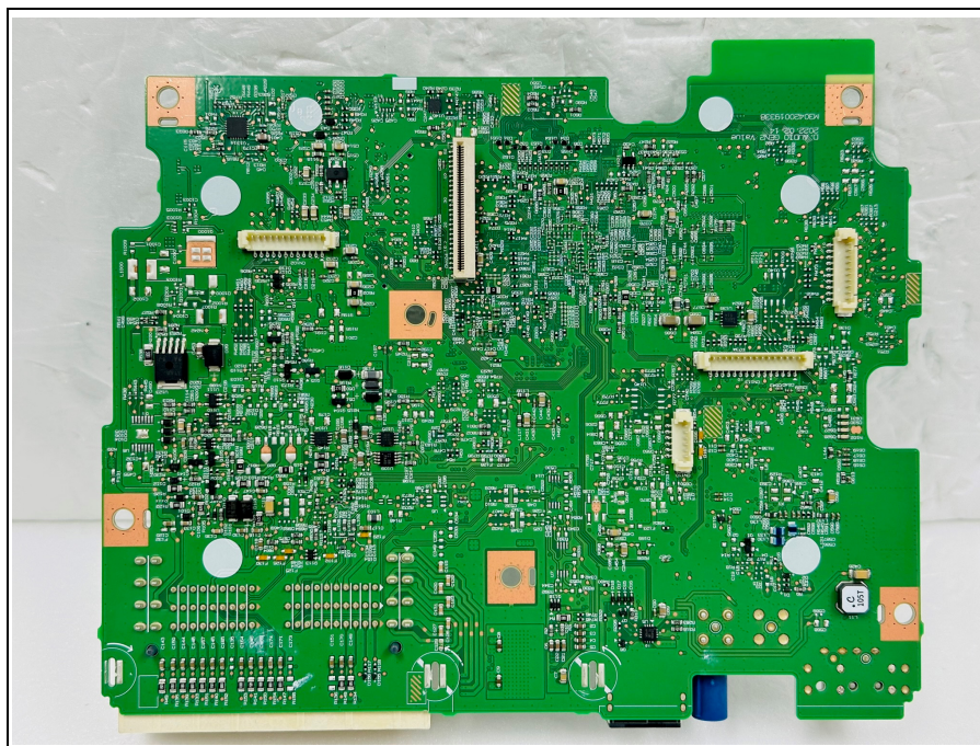
Bottom view of Sub1 PCB
