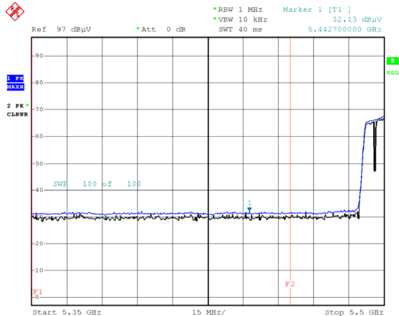
Average Reading (802.11n_VHT40, Ch.102, X-V)
