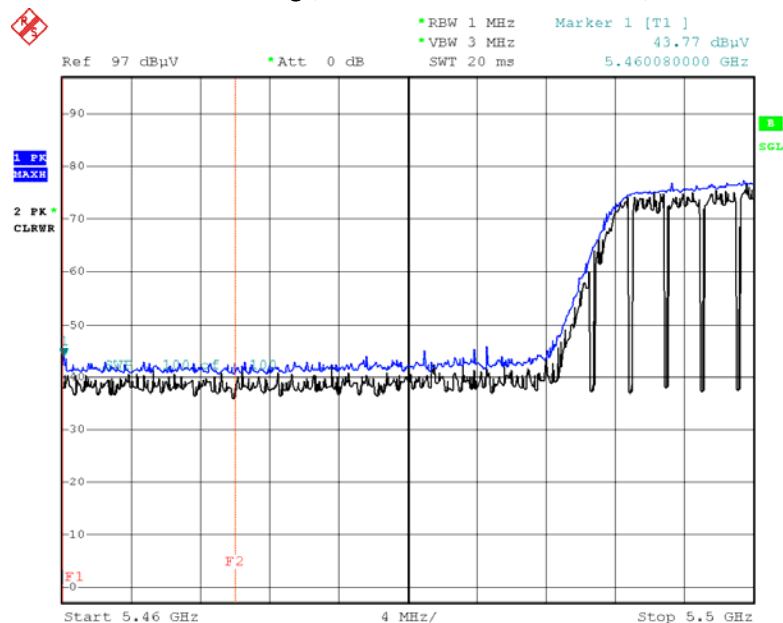
Peak Reading (802.11n_VHT40 Ch.102, X-V)
