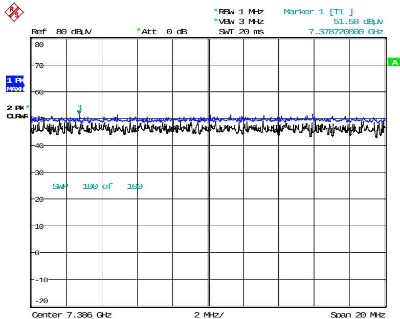
Radiated Spurious Emissions plot – Peak Reading (802.11b, Ch.11 3rd Harmonic)
