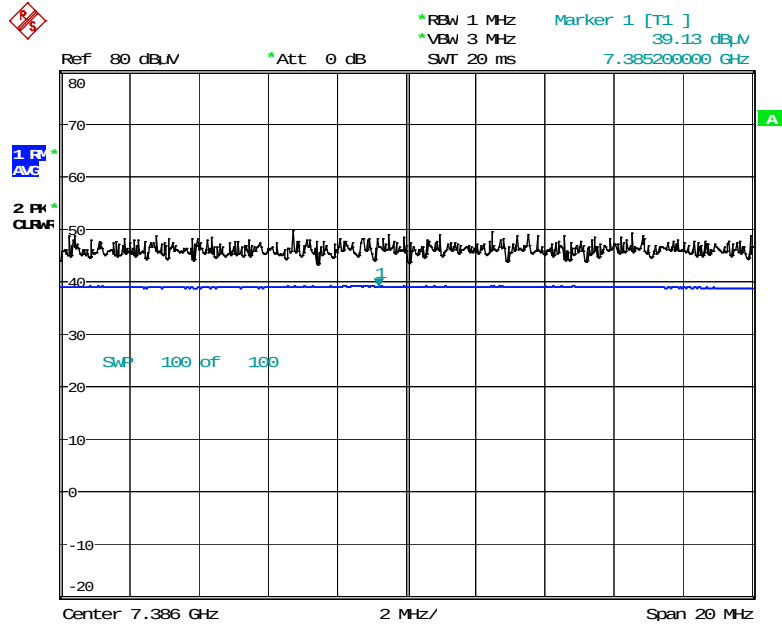
Radiated Spurious Emissions plot – Average Reading (802.11b, Ch.11 3rd Harmonic)
