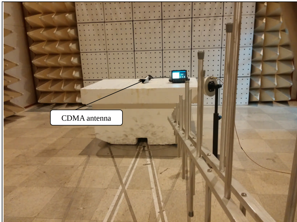
Photo of Field Strength & Spurious Emission Test(CDMA)
