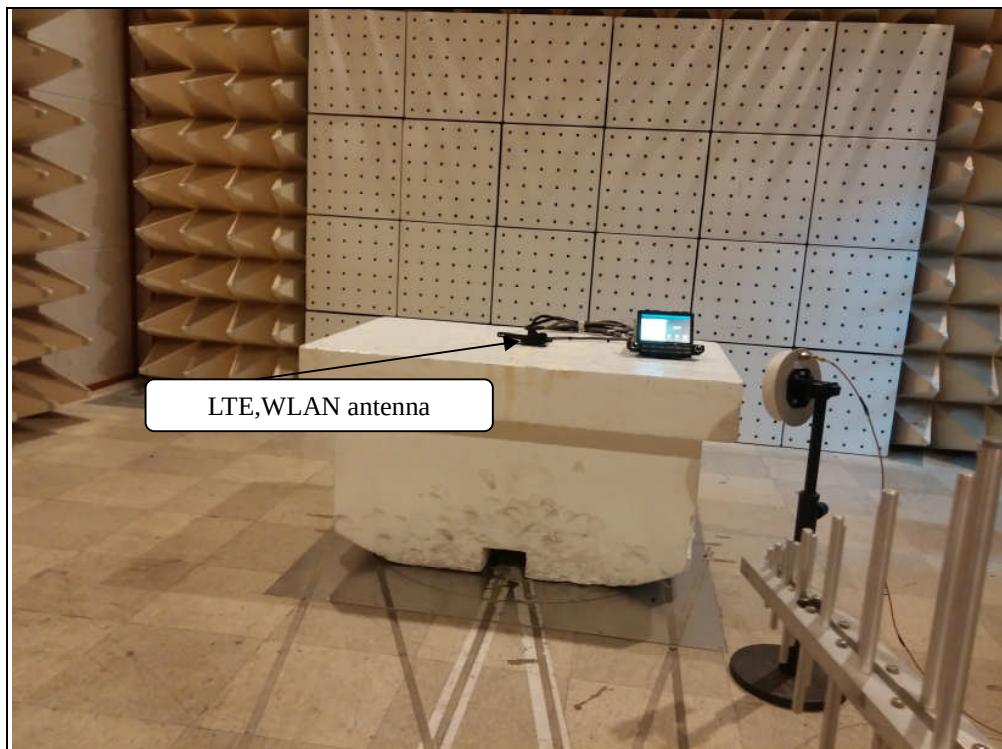
Photo of Field Strength & Spurious Emission Test(LTE,WLAN)
