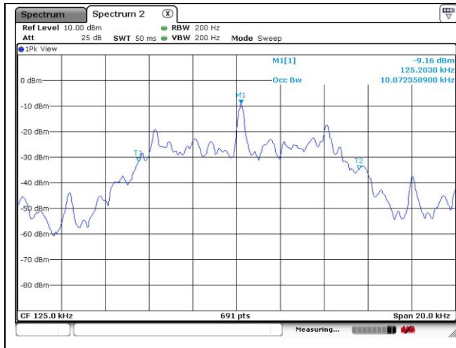
DRV Antenna
