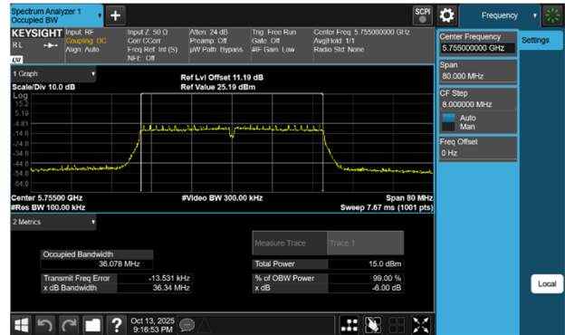
Bandwidth 40M, 802.11ac(VHT40) Ch.151
