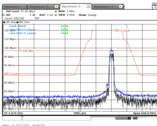
Peak Result (802.11ac_VHT20, Ch.161, X-V)
