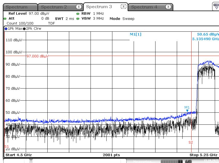
Peak Result (802.11ac80_ MCS0, Ch. 42, X-V)
