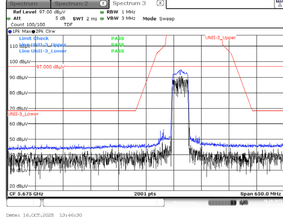
Peak Result (802.11ac_VHT80, Ch.155, X-V)
