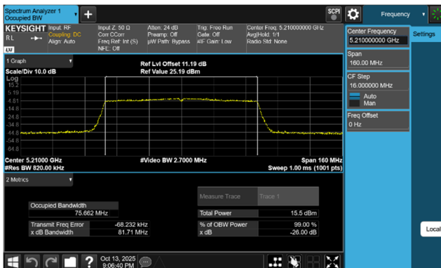
Bandwidth 80M, 802.11ac(VHT80) Ch.42
