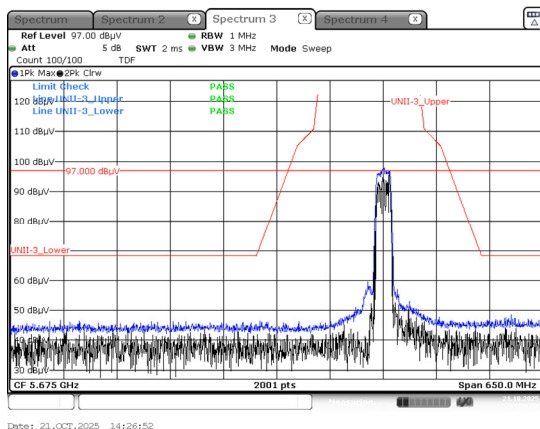
Peak Result (802.11ac_VHT40, Ch.159, X-V)
