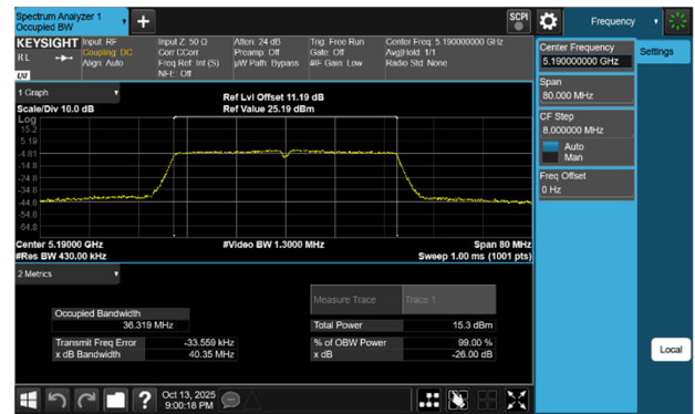
Bandwidth 40M, 802.11n(HT40) Ch.38
