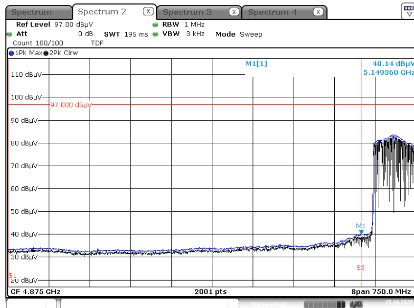
Average Result (802.11ac80_ MCS0, Ch. 42, X-V)
