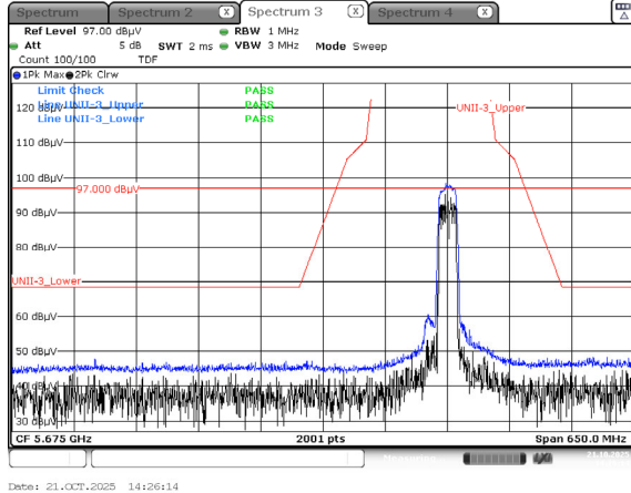
Peak Result (802.11n_HT40, Ch.159, X-V)
