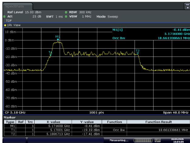
Ant.1_Low Channel (5 180 MHz)_0 RU
