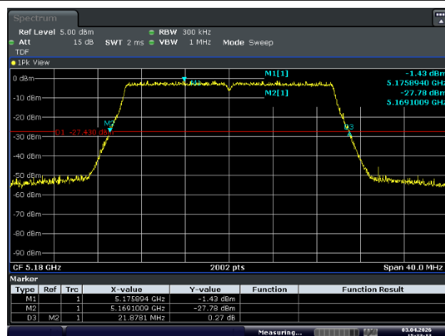
Ant.2_Low Channel (5 180 MHz)
