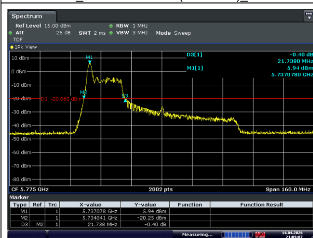
Ant.1_Middle Channel (5 775 MHz)_0 RU
