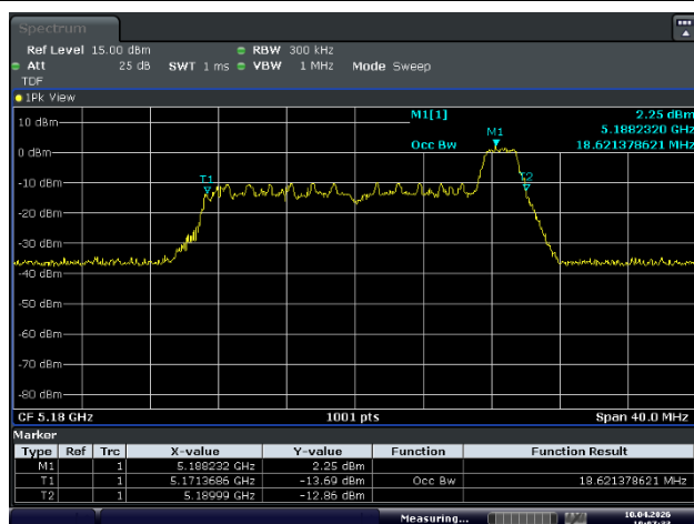
Ant.1_Low Channel (5 180 MHz)_8 RU
