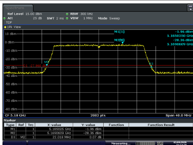
Ant.1_Low Channel (5 180 MHz)
