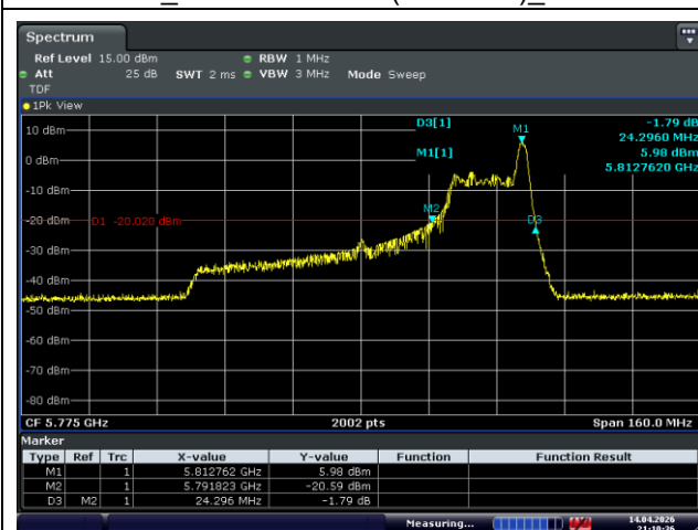
Ant.1_Middle Channel (5 775 MHz)_36 RU
