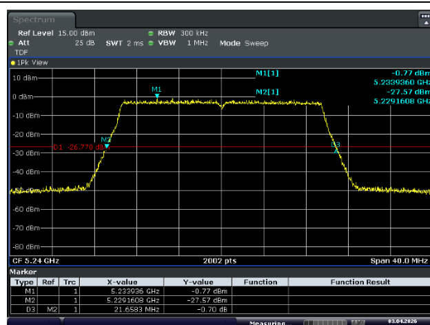
Ant.2_High Channel (5 240 MHz)
