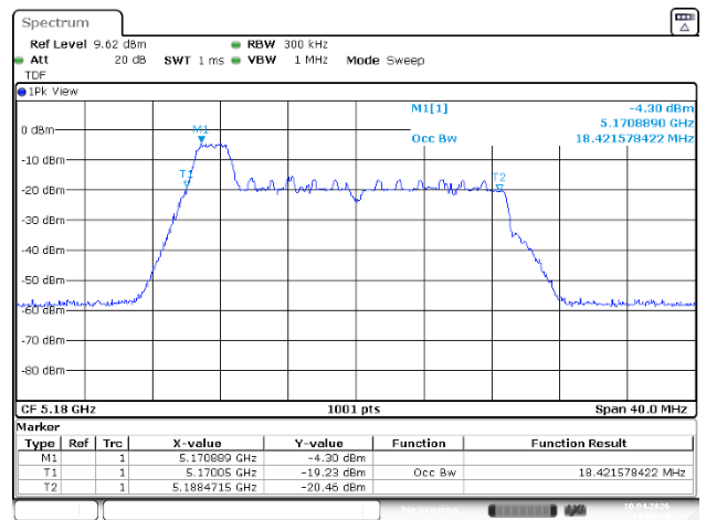
Ant.2_Low Channel (5 180 MHz)_0 RU
