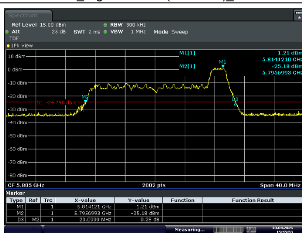
Ant.1_High Channel (5 805 MHz)_8 RU
