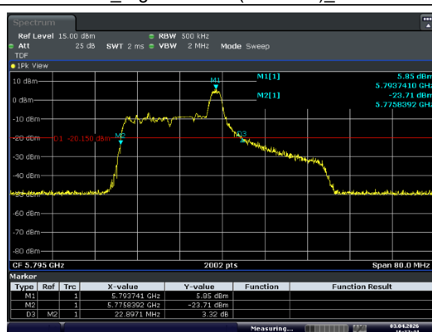
Ant.2_High Channel (5 795 MHz)_8 RU
