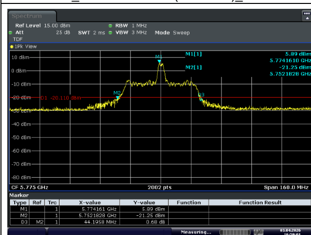
Ant.1_Middle Channel (5 775 MHz)_18 RU
