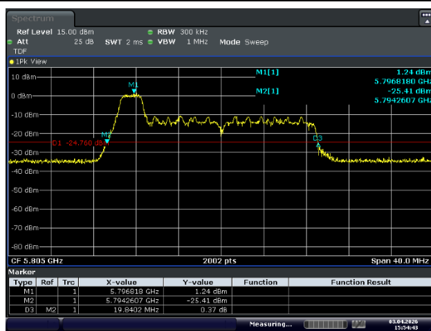
Ant.1_High Channel (5 805 MHz)_0 RU
