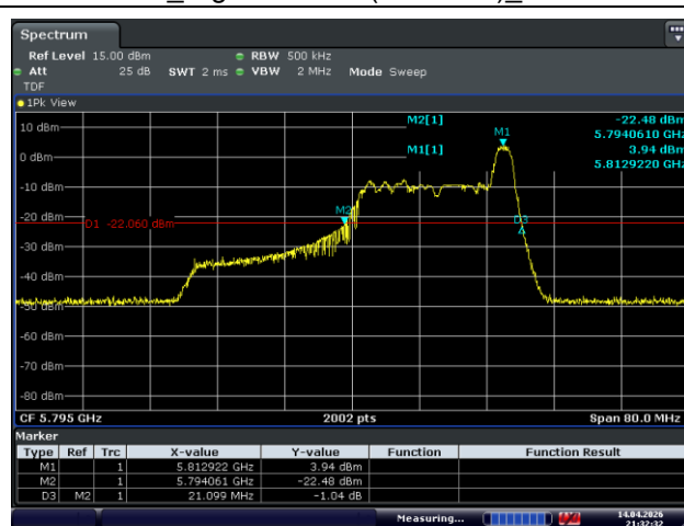
Ant.2_High Channel (5 795 MHz)_17 RU
