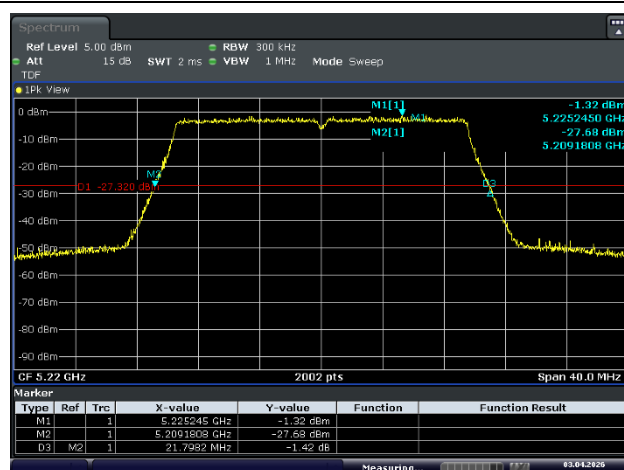
Ant.2_Middle Channel (5 220 MHz)
