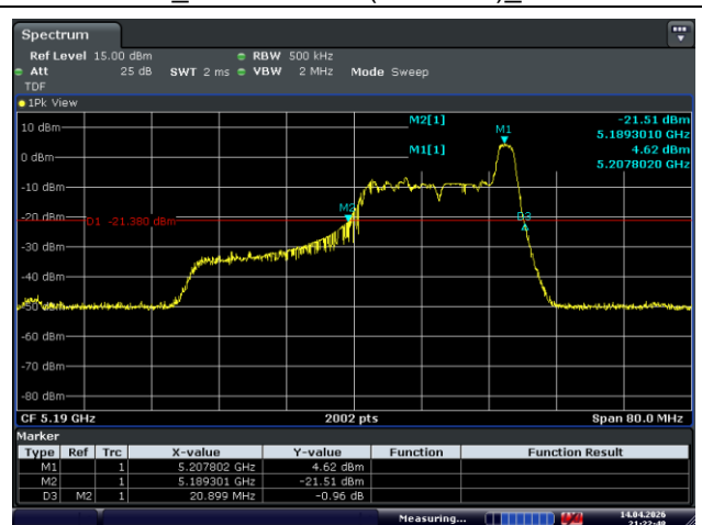
Ant.2_Low Channel (5 190 MHz)_17 RU
