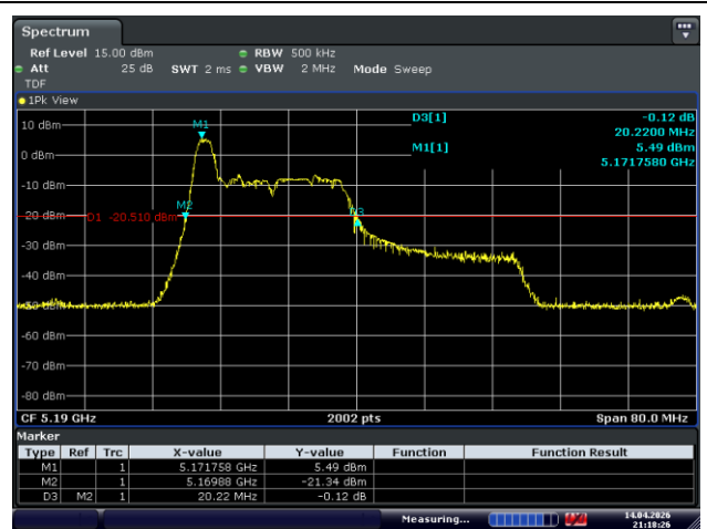
Ant.2_Low Channel (5 190 MHz)_0 RU
