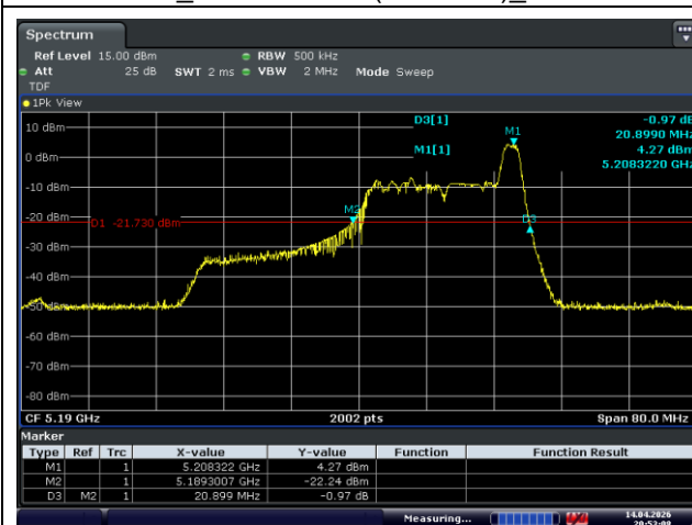
Ant.1_Low Channel (5 190 MHz)_17 RU
