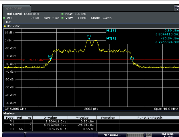
Ant.1_High Channel (5 805 MHz)_4 RU
