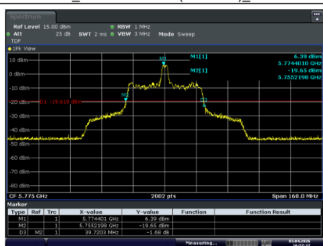
Ant.2_Middle Channel (5 775 MHz)_18 RU
