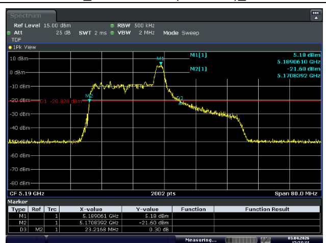
Ant.2_Low Channel (5 190 MHz)_8 RU
