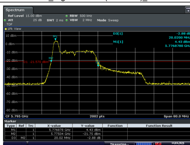
Ant.2_High Channel (5 795 MHz)_0 RU
