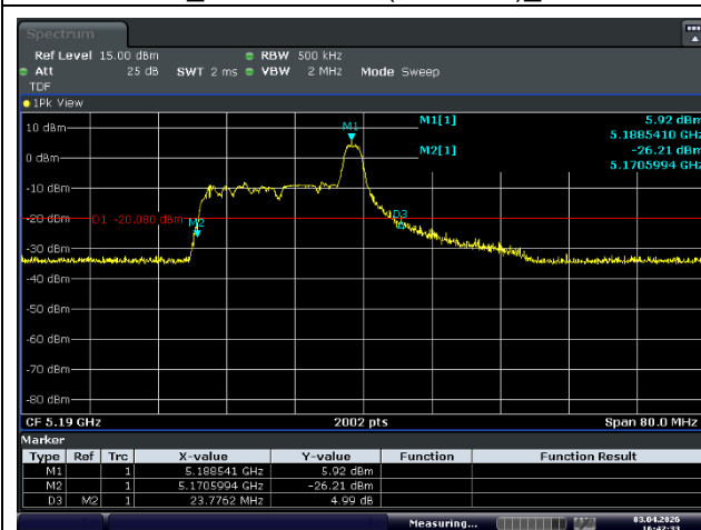
Ant.1_Low Channel (5 190 MHz)_8 RU
