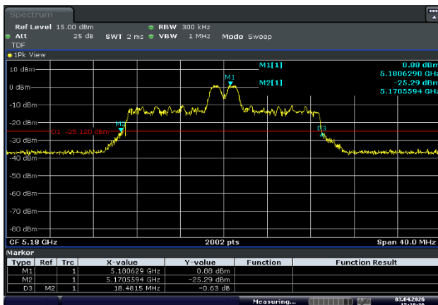
Ant.1_Low Channel (5 180 MHz)_8 RU
