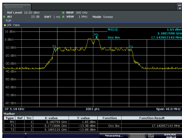
Ant.1_Low Channel (5 180 MHz)_4 RU
