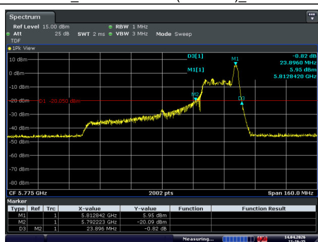
Ant.2_Middle Channel (5 775 MHz)_36 RU
