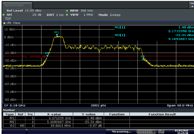
Ant.1_Low Channel (5 180 MHz)_4 RU
