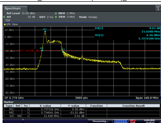
Ant.2_Middle Channel (5 775 MHz)_0 RU
