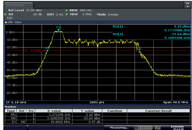
Ant.2_Low Channel (5 180 MHz)_4 RU
