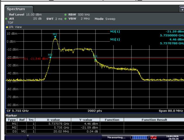
Ant.1_Low Channel (5 755 MHz)_0 RU
