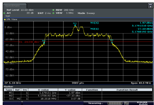
Ant.2_Low Channel (5 180 MHz)_8 RU
