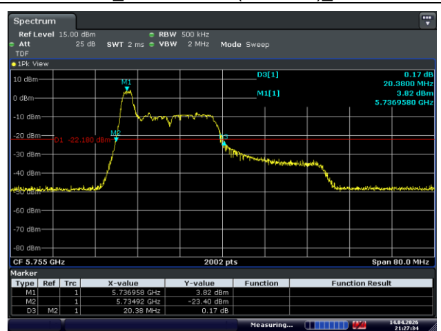
Ant.2_Low Channel (5 755 MHz)_0 RU
