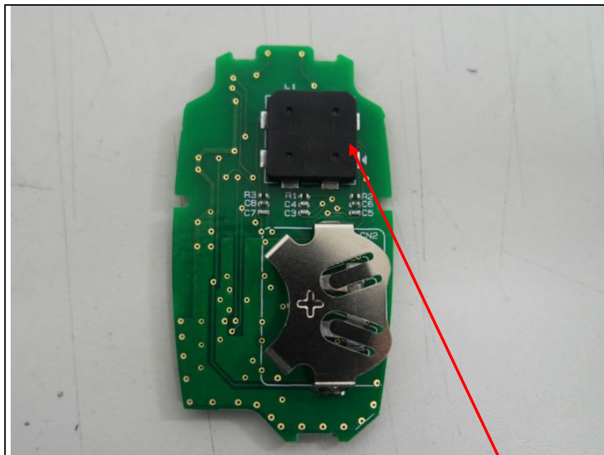
Rx Antenna (with built-in IC)
