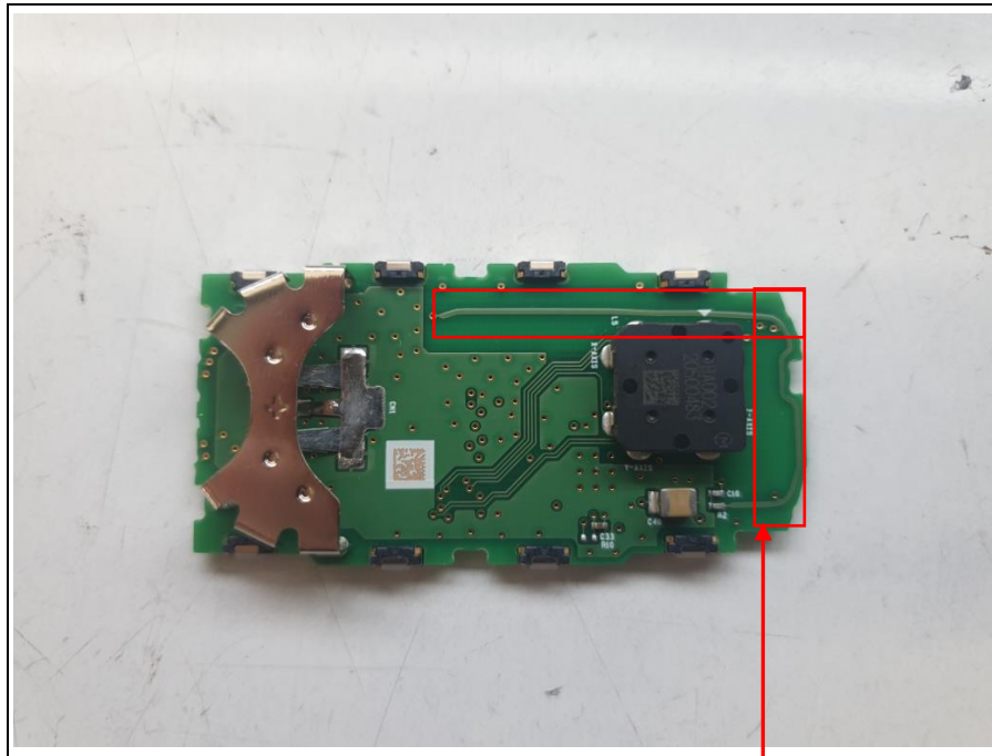
433MHz PCB Pattern Antenna
