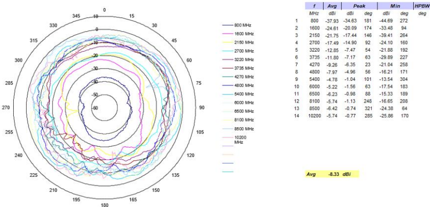
2D 측정_ E1 Plane
