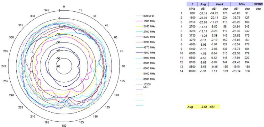
2D 측정_ E2 Plane
