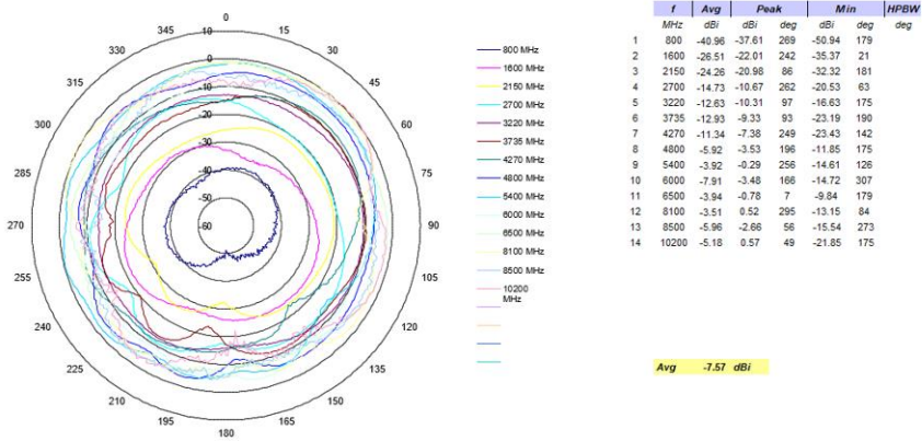
2D 측정_ H Plane
