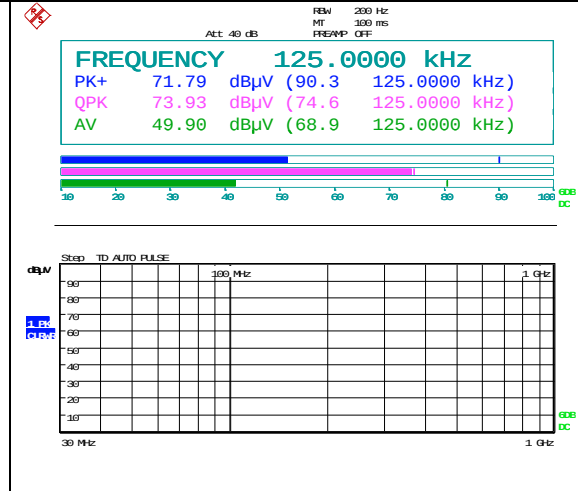
AST Antenna
