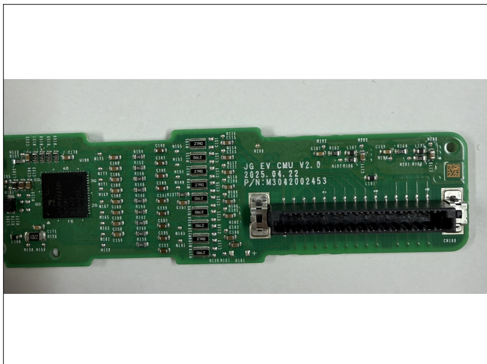
Top view of PCB(Right)
