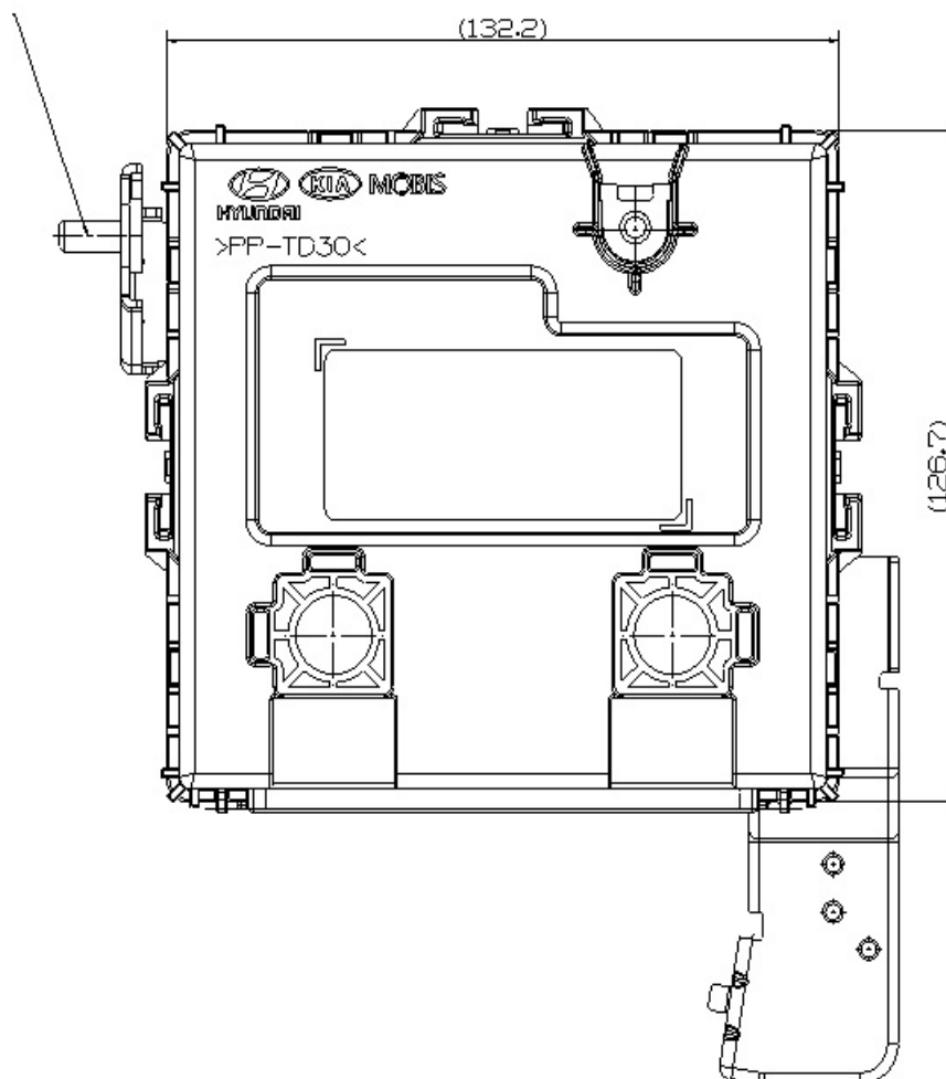
Front view (1:1)
