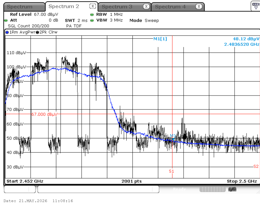
Radiated Restricted Band Edges plot – Average Result (802.11n(HT20) MCS0, Ch.11, X-V)
