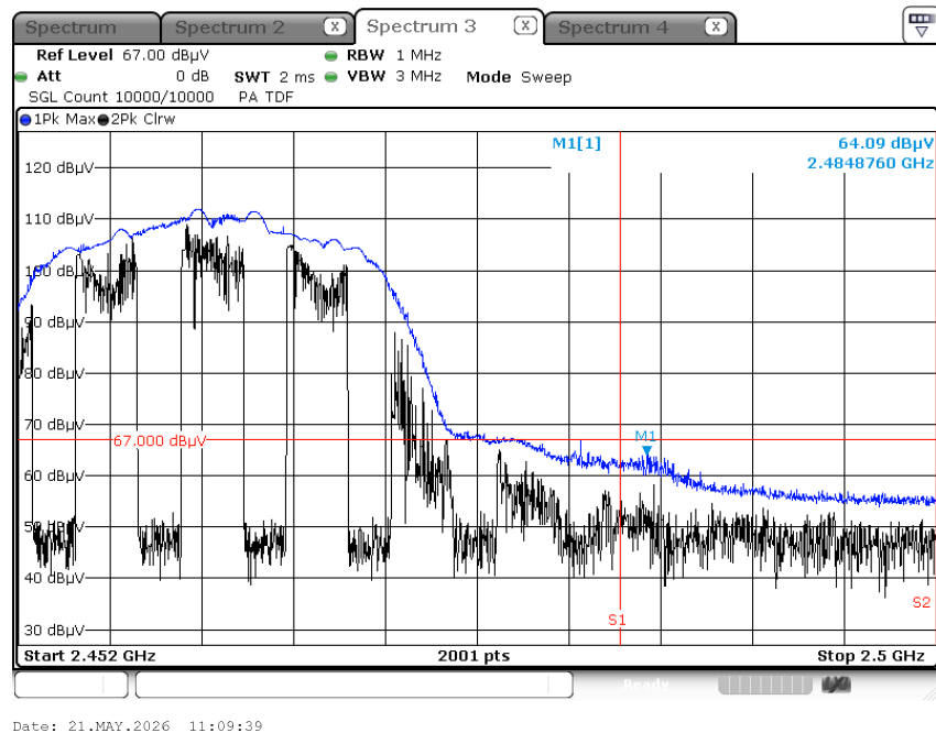
Radiated Restricted Band Edges plot – Peak Result (802.11n(HT20) MCS0, Ch.11, X-V)
