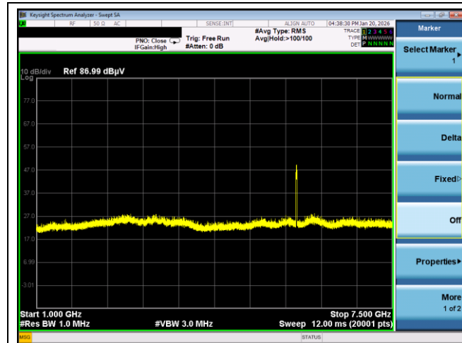
1 GHz ~ 7.5 GHz
