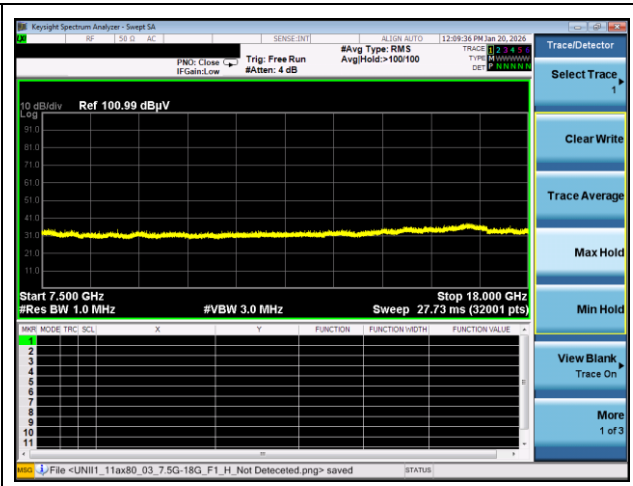
7.5 GHz ~ 18 GHz
