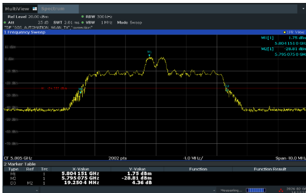
Ant.1_High Channel (5 805 MHz)_8 RU
