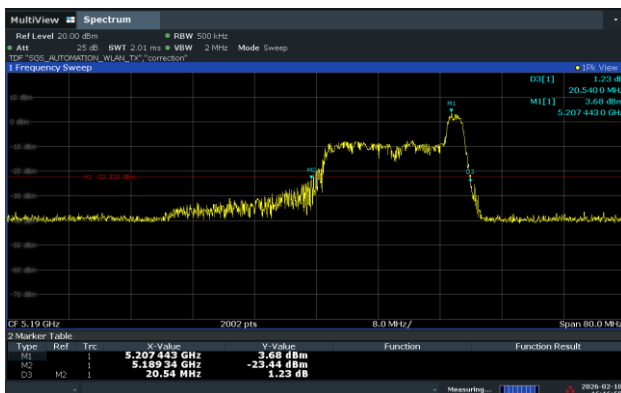
Ant.1_Low Channel (5 190 MHz)_17 RU
