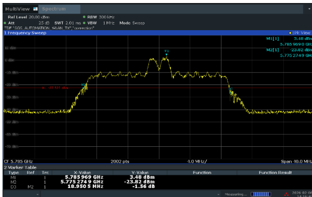
Ant.1_Middle Channel (5 785 MHz)_8 RU
