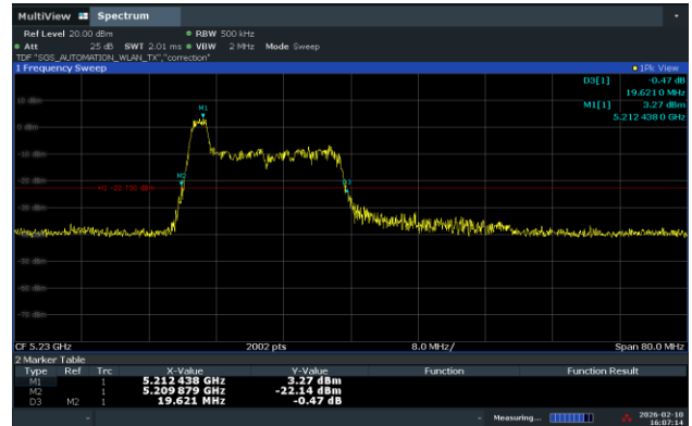
Ant.2_High Channel (5 230 MHz)_8 RU
