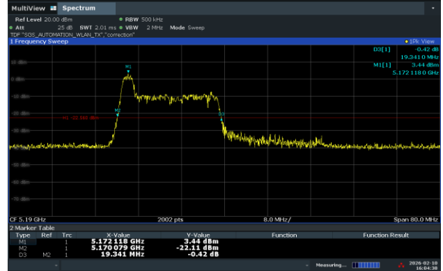
Ant.2_Low Channel (5 190 MHz)_8 RU
