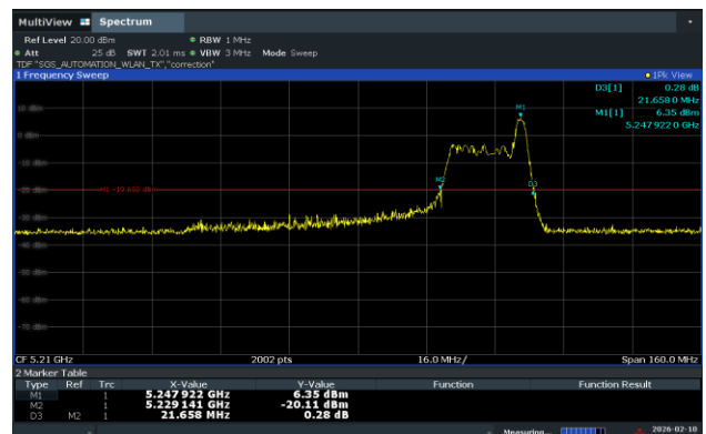
Ant.2_Middle Channel (5 210 MHz)_36 RU
