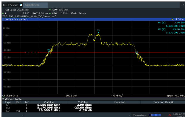
Ant.1_Low Channel (5 180 MHz)_8 RU
