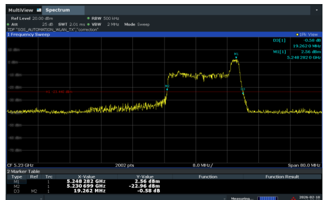
Ant.2_High Channel (5 230 MHz)_17 RU
