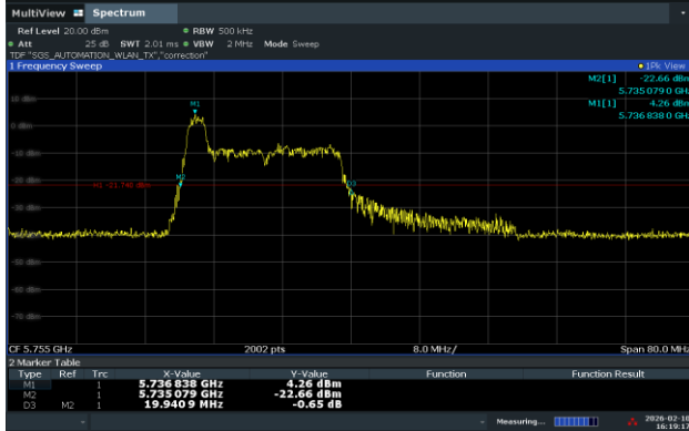
Ant.1_Low Channel (5 755 MHz)_8 RU
