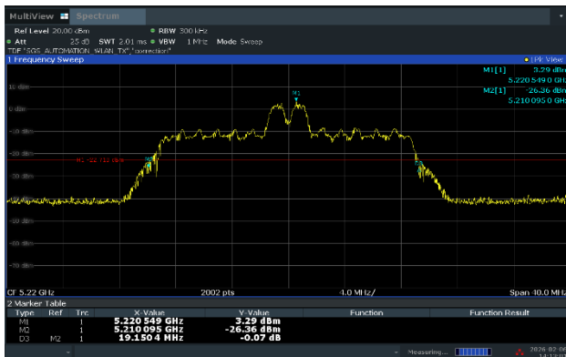
Ant.1_Middle Channel (5 220 MHz)_8 RU
