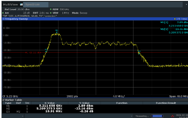
Ant.1_Middle Channel (5 220 MHz)_4 RU
