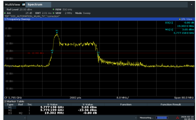
Ant.2_High Channel (5 795 MHz)_8 RU
