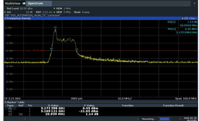
Ant.2_Middle Channel (5 210 MHz)_18 RU
