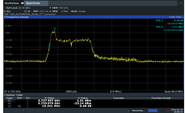
Ant.2_Low Channel (5 755 MHz)_8 RU
