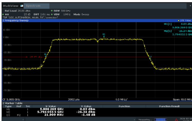
Ant.1_High Channel (5 805 MHz)
