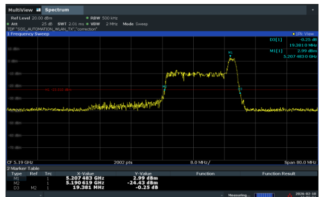
Ant.2_Low Channel (5 190 MHz)_17 RU
