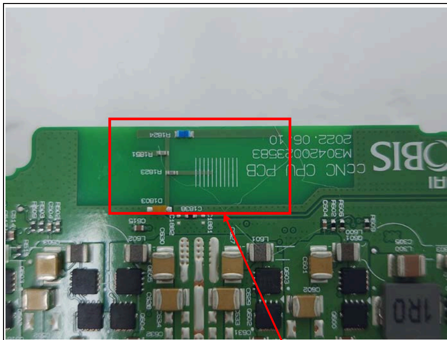
WiFi 2.4GHz and 5GHz Core1 Dual Antenna
