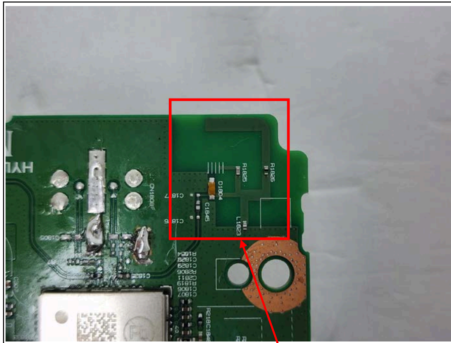
BT+ WiFi 5GHz Core0 Antenna
