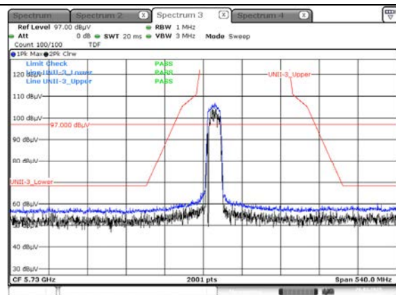
Peak Result (802.11n_HT20, Ch.149, X-H)
