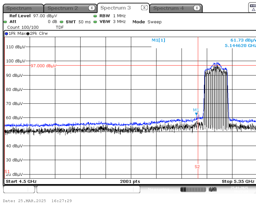
Peak Result (802.11 ac_VHT80_ MCS0, Ch.42, X-H)
