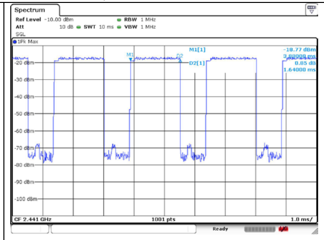
Operation Mode: 8DPSK
