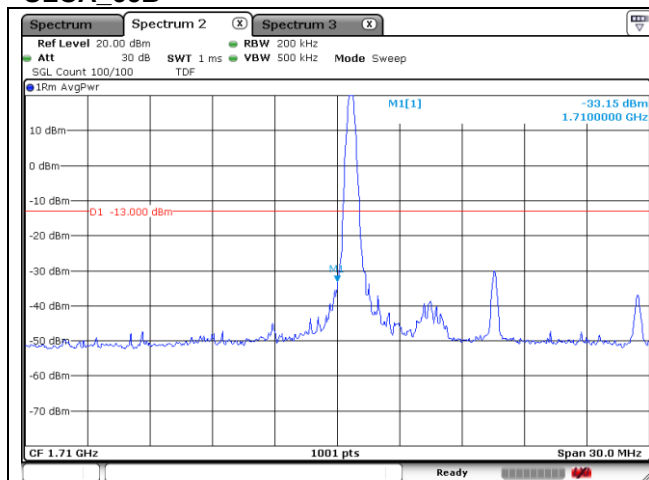
PCC 5 MHz + SCC 10 MHz QPSK-Low Channel – 1 RB
