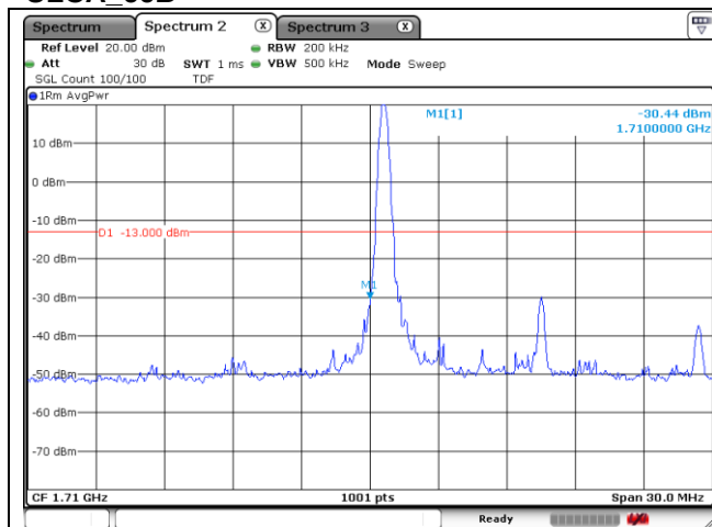
PCC 10 MHz + SCC 5 MHz 16QAM-Low Channel – 1 RB
