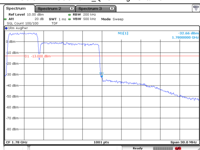
PCC 5 MHz + SCC 10 MHz QPSK-High Channel – Full RB
