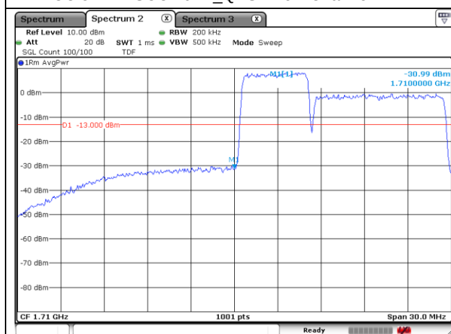
PCC 5 MHz + SCC 10 MHz QPSK-Low Channel – Full RB
