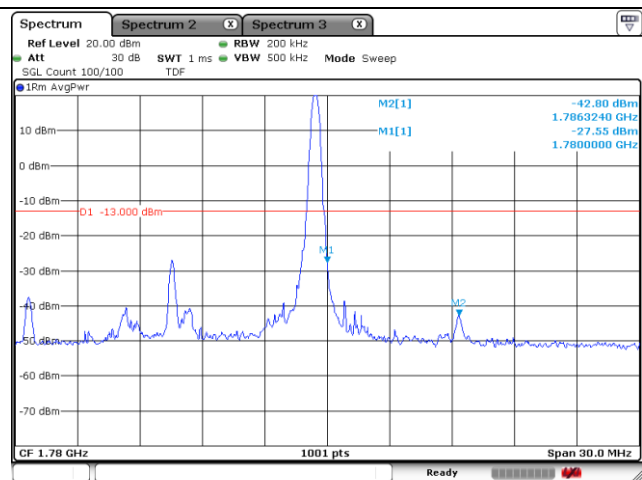
PCC 5 MHz + SCC 10 MHz QPSK-High Channel – 1 RB
