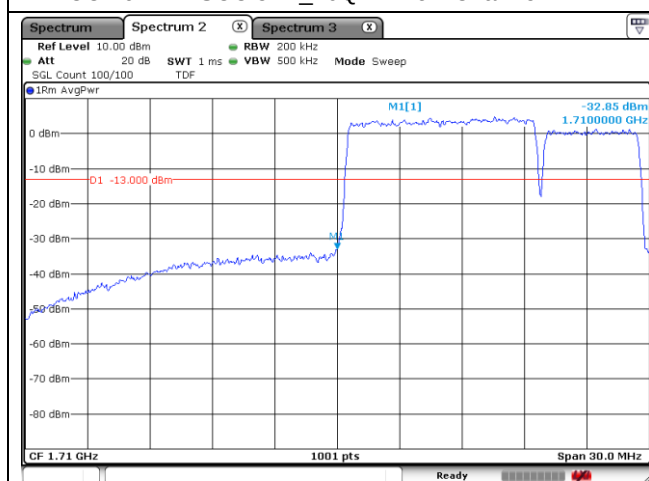
PCC 10 MHz + SCC 5 MHz 16QAM-Low Channel – Full RB
