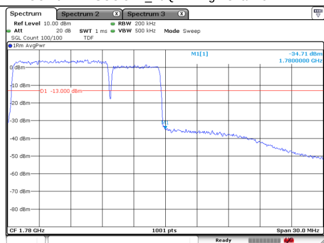
PCC 10 MHz + SCC 5 MHz 16QAM-High Channel – Full RB
