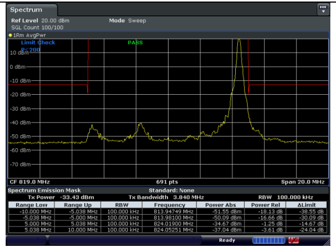
QPSK Middle Channel - 1 RB_High
