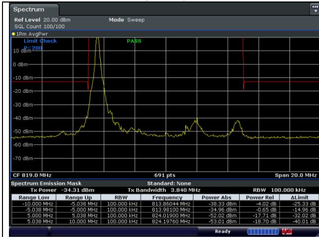
QPSK Middle Channel - 1 RB_Low
