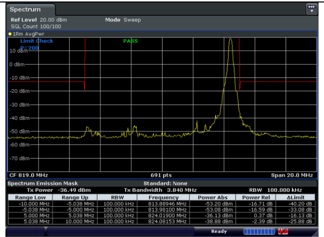
16QAM Middle Channel - 1 RB_High
