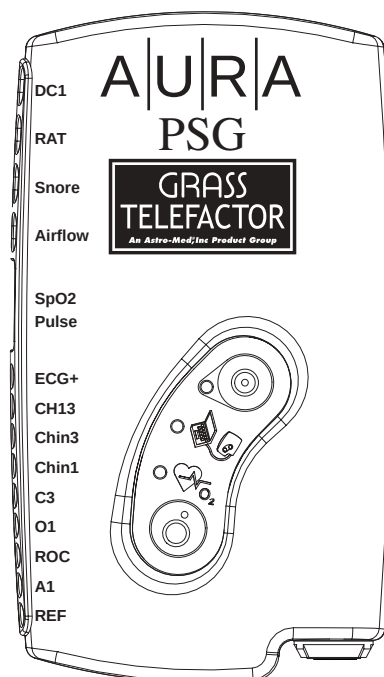
Figure 4-2: Amplifier Unit Controls
