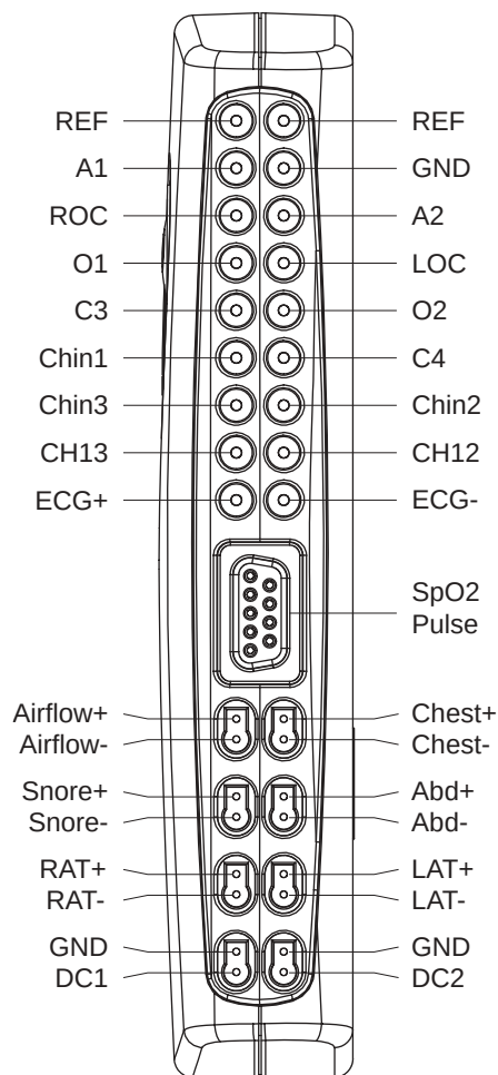
Figure 3-4: Amplifier Unit inputs
