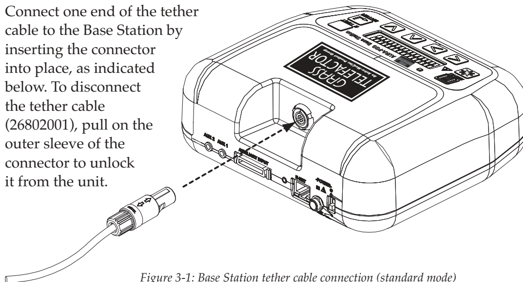
Figure 3-1: Base Station tether cable connection (standard mode)
