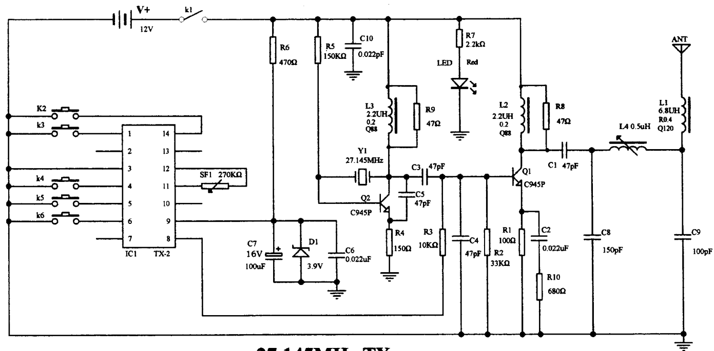
27.145MHz TX
