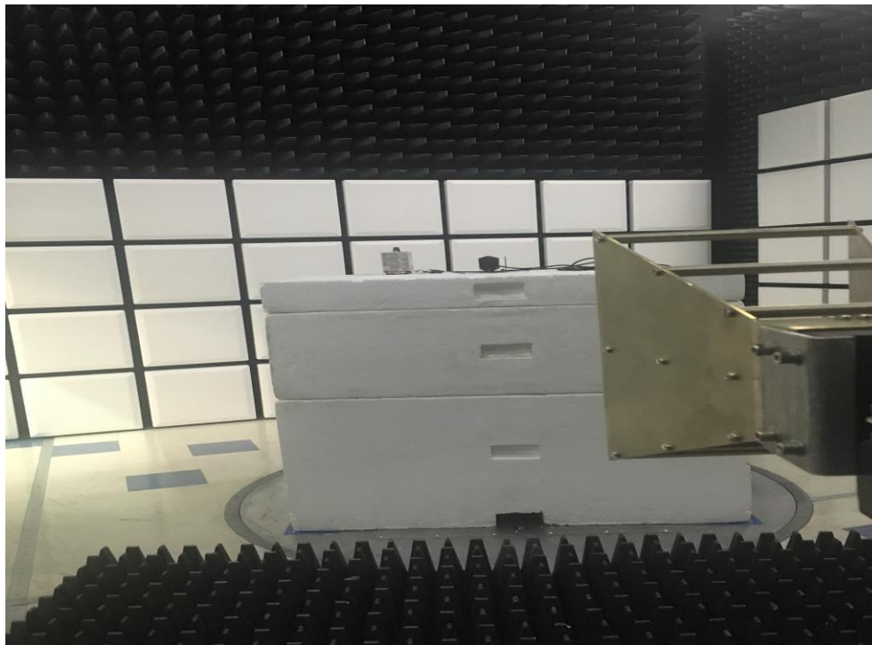
Radiated measurement from 1-18 GHz
