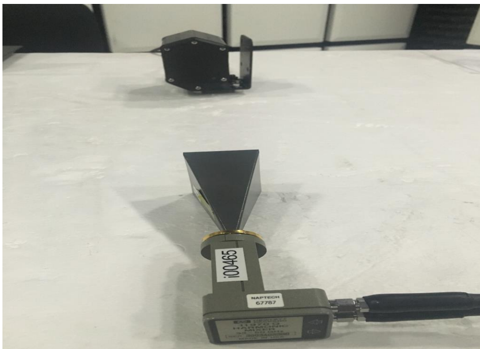
Radiated measurement from 33-50 GHz
