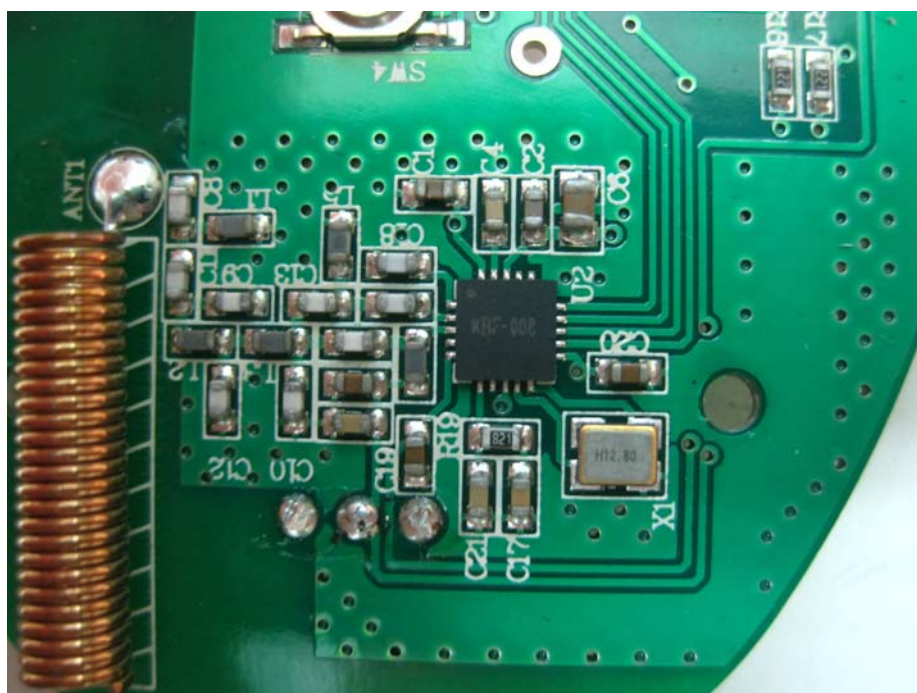
Close View of the PCB
