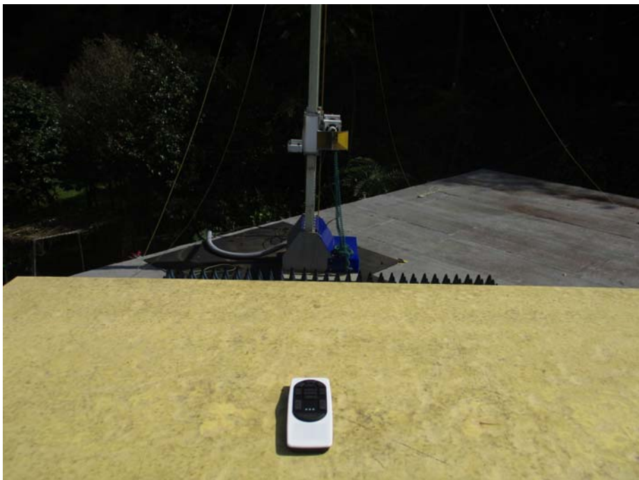
Above 1 GHz (The height of testing table is 1.5m)
