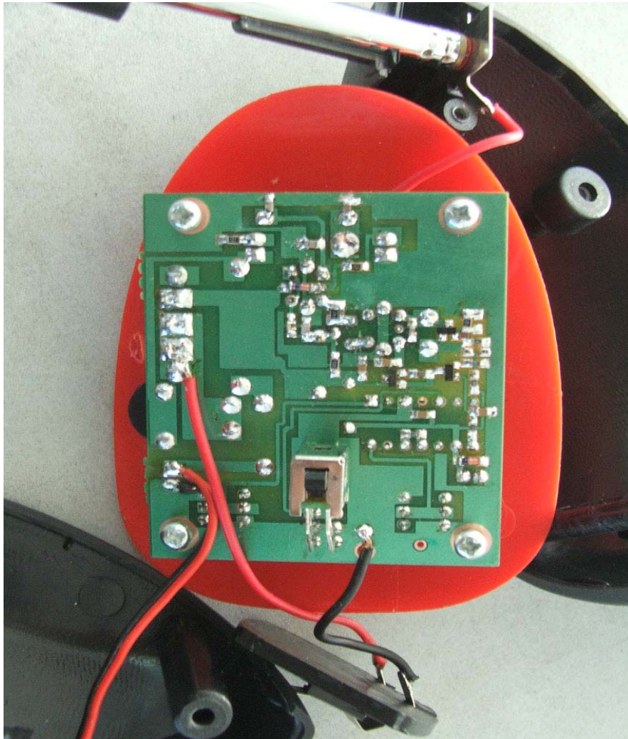
Transmitter - Main Board Soldered View
