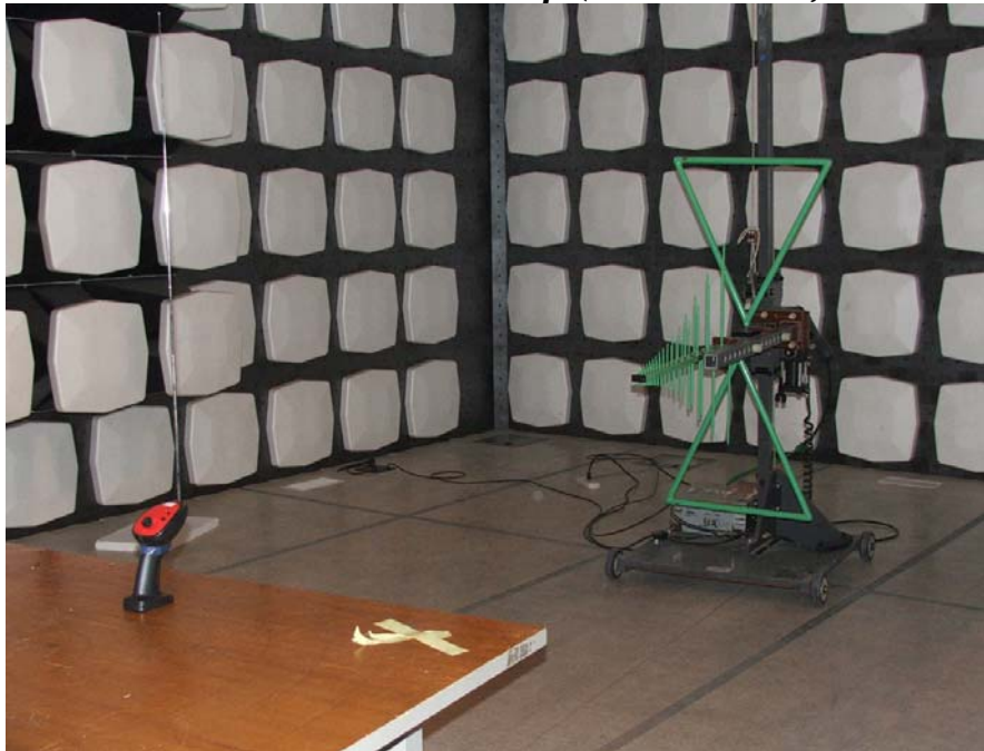
RADIATED EMISSION TEST Set-up (Transmitter, Vertical)
