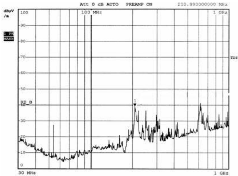
Horizontal Radiated Emission Plot (Receiver)
