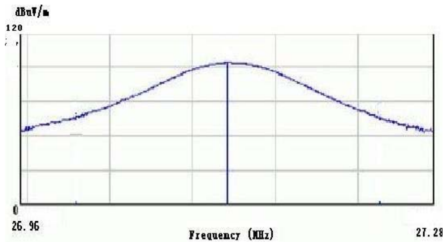
Field Strength within the Band – Vertical View
