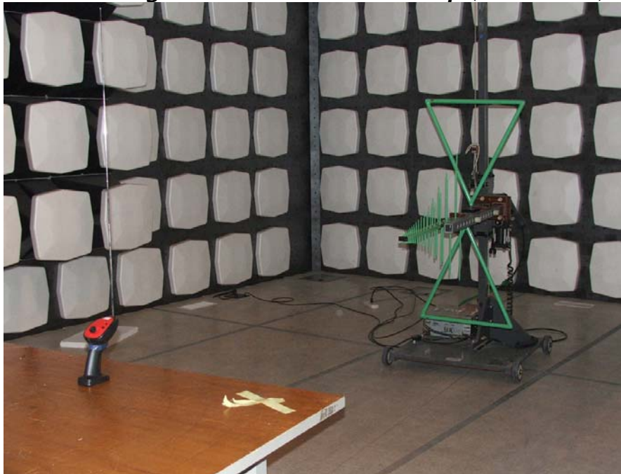
Field Strength within Band Test Set-up (Vertical)
