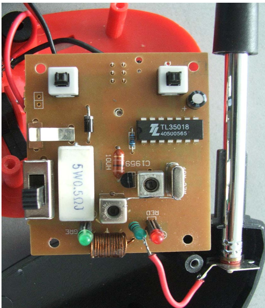
Transmitter - Main Board Component View
