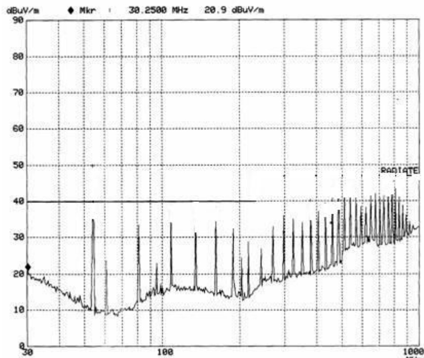
Vertical Radiated Emission Plot (Transmitter)
