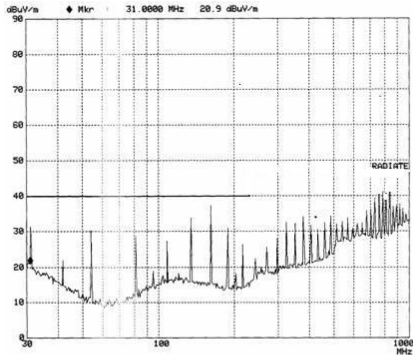
Horizontal Radiated Emission Plot (Transmitter)
