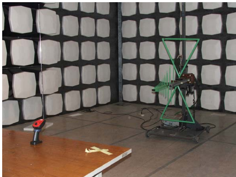
RADIATED EMISSION ((Transmitter) V)
