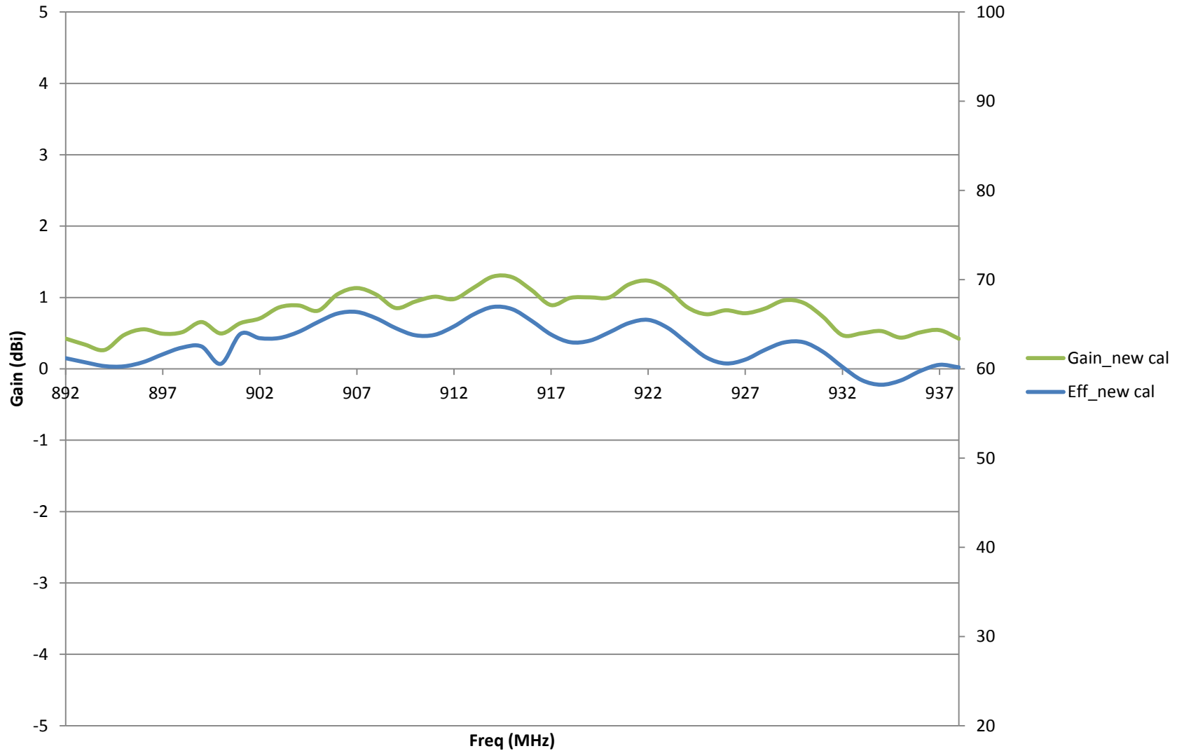
Antenna Proto 1
