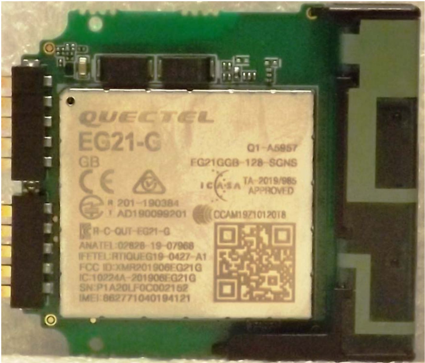
Figure E22.2 – Internal – PCB Bottom
